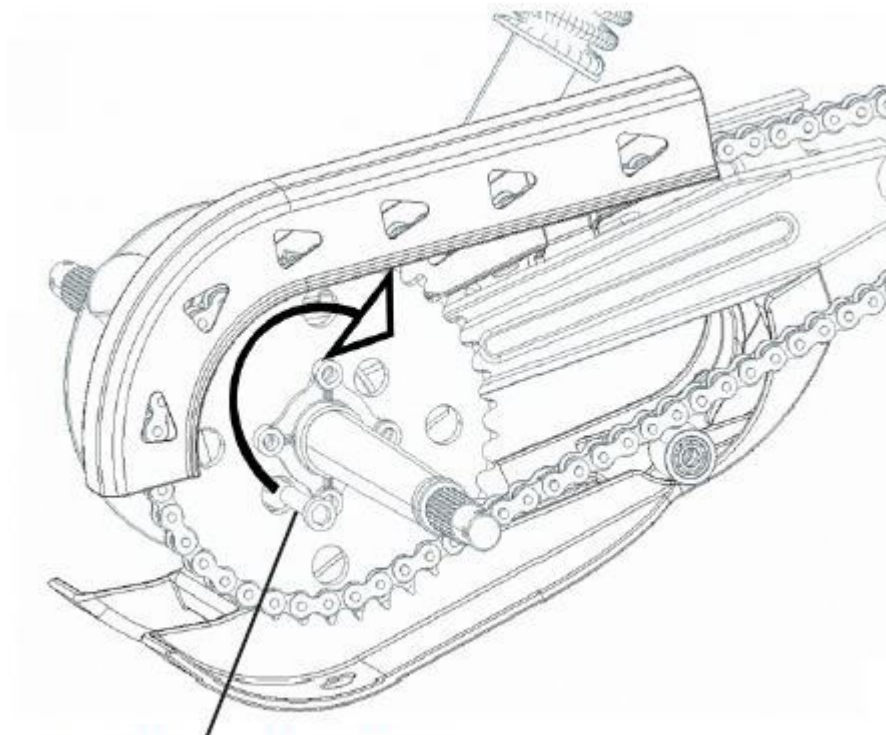
Kedjejusteringsbult M10x60
