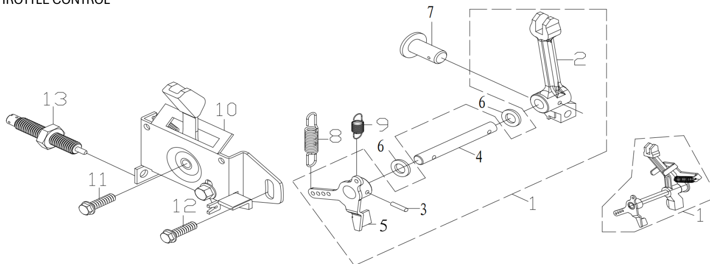
FIGUR E18 - THROTTLE CONTROL
