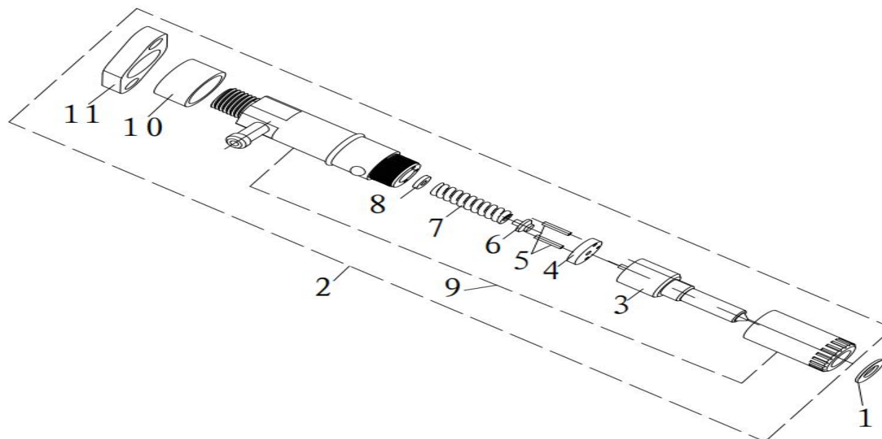
FIGUR E17 - FUEL INJECTION ASSY
