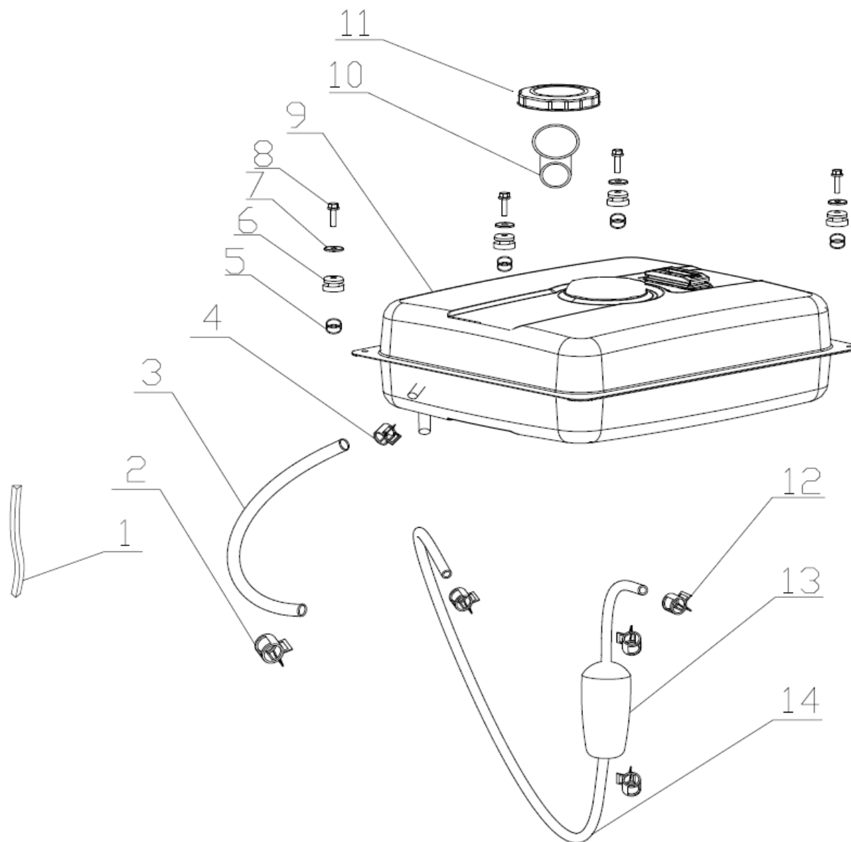
FIGUR 2 - FUEL TANK ASSEMBLY
