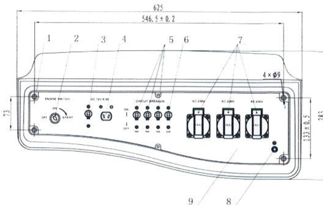
FIGUR 5 – KONTROLLPANEL / CONTROL PANEL
