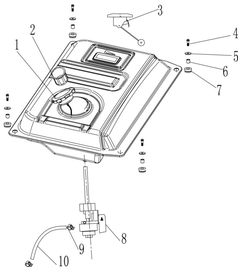
FIGUR 2 - BENSINTANK / FUEL TANK
