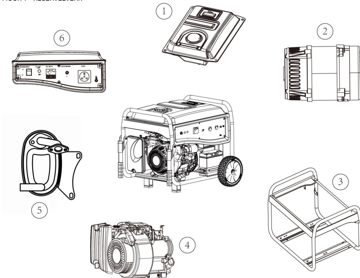
FIGUR 1 – RESERVELVERK
