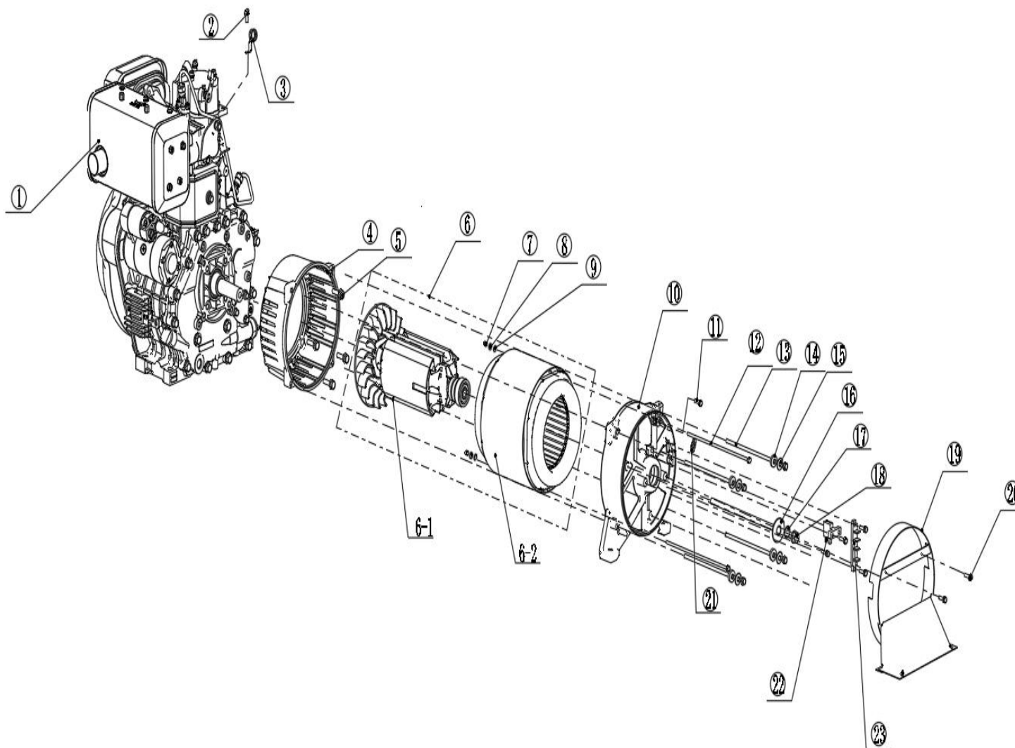
FIGUR 3 – ALTERNATOR
