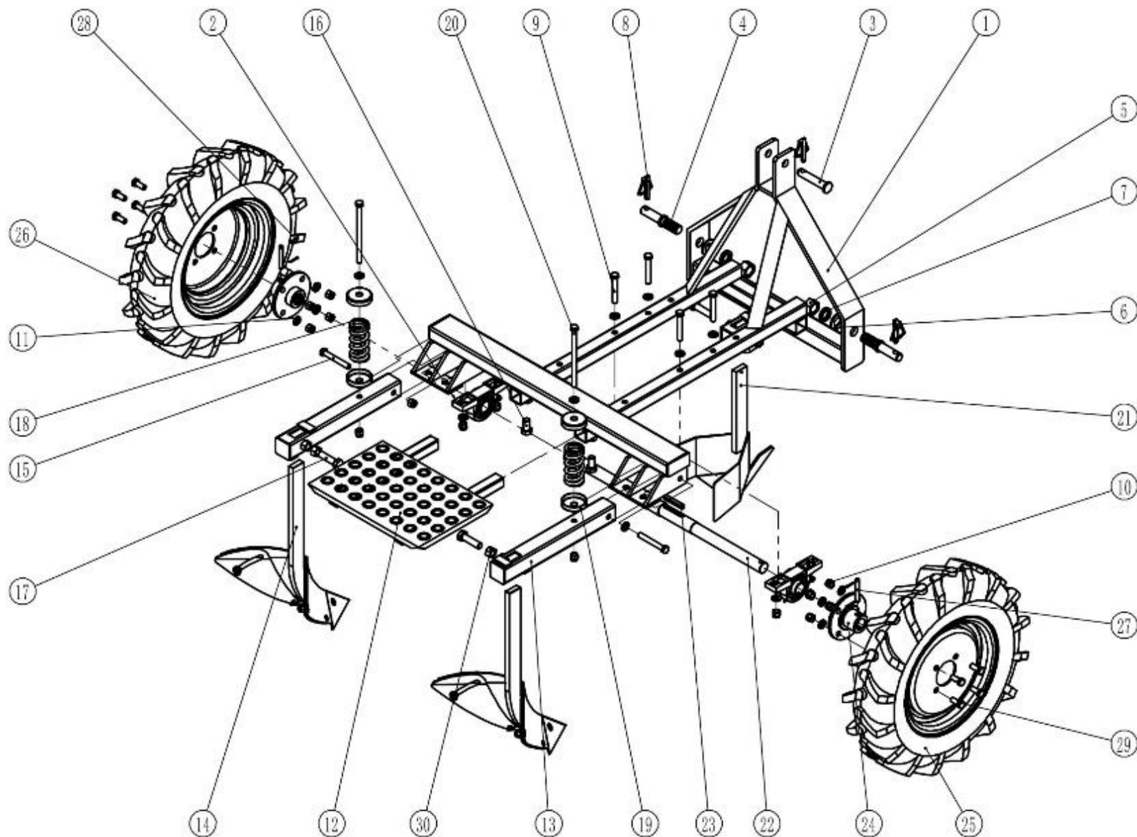
FIGUR 3 - Main welding assembly
