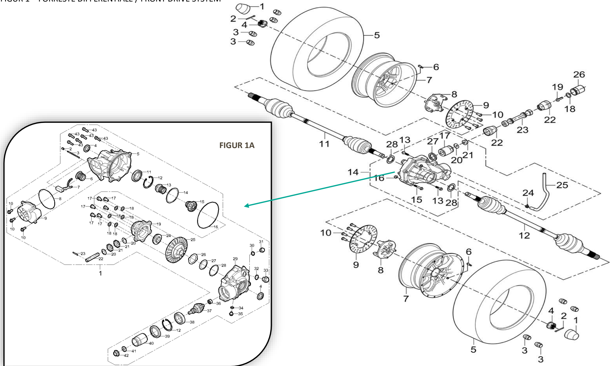
FIGUR 1 – FORRESTE DIFFERENTIALE / FRONT DRIVE SYSTEM
