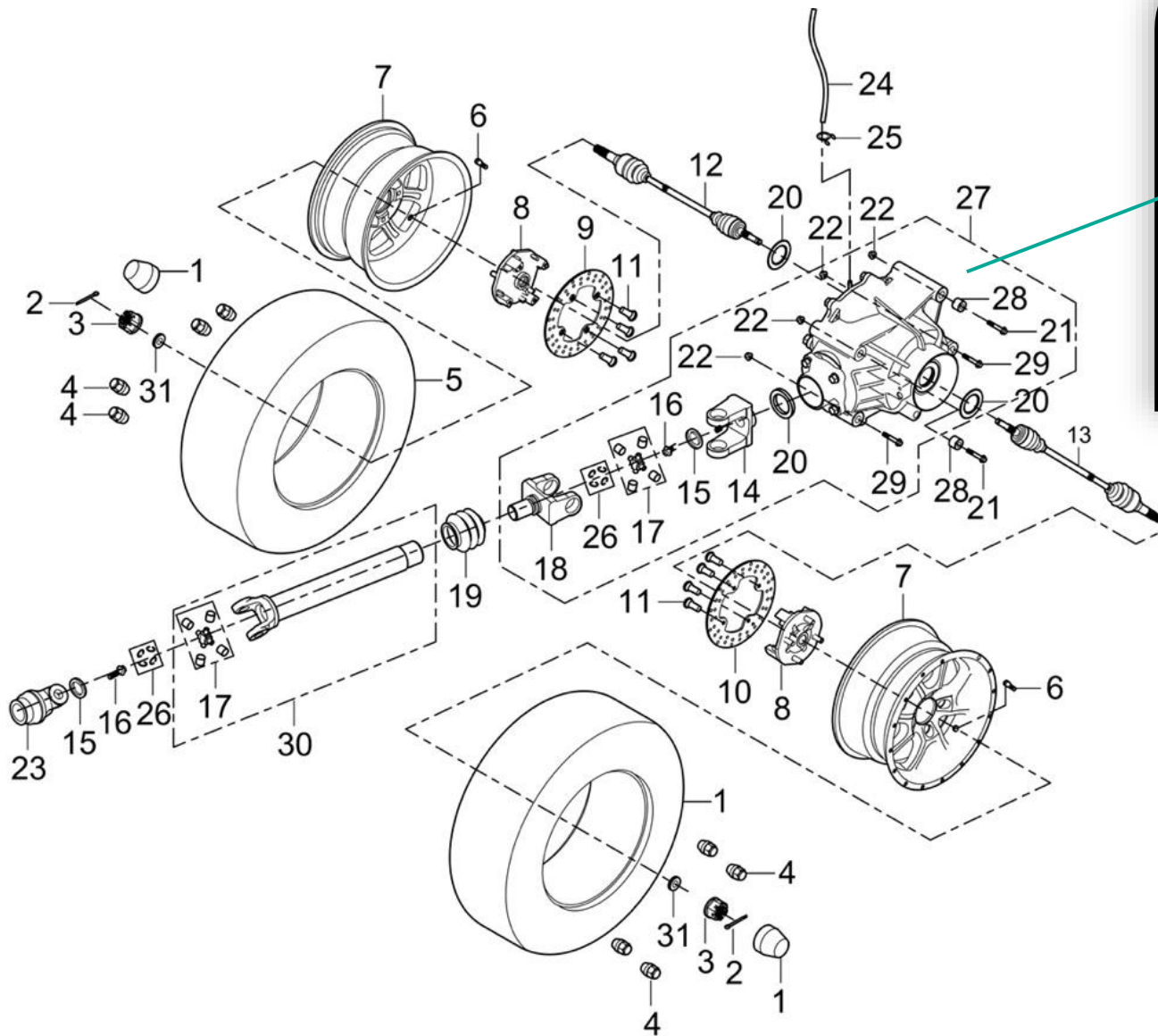
FIGUR 2 – BAGERSTE DIFFERENTIALE / REAR DRIVE SYSTEM
