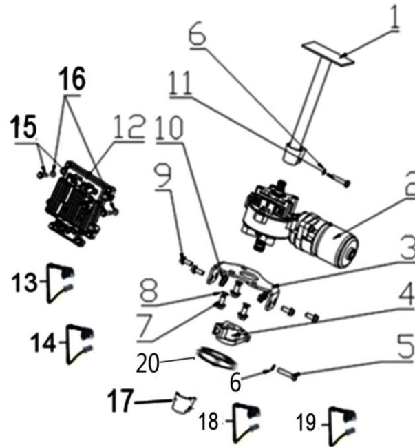
FIG 22 – SERVOSTYRING / EPS
