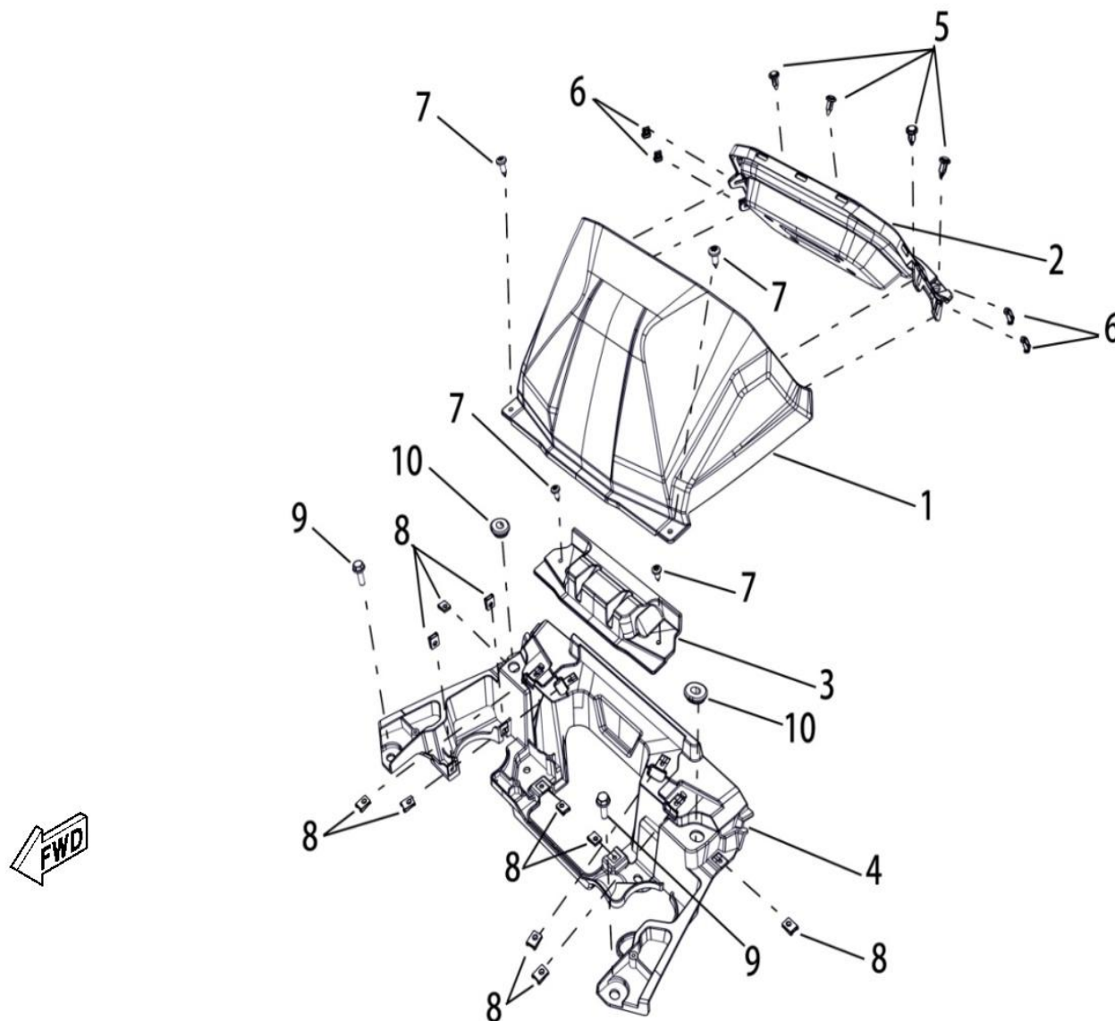
FIGUR 7 - FENDER
