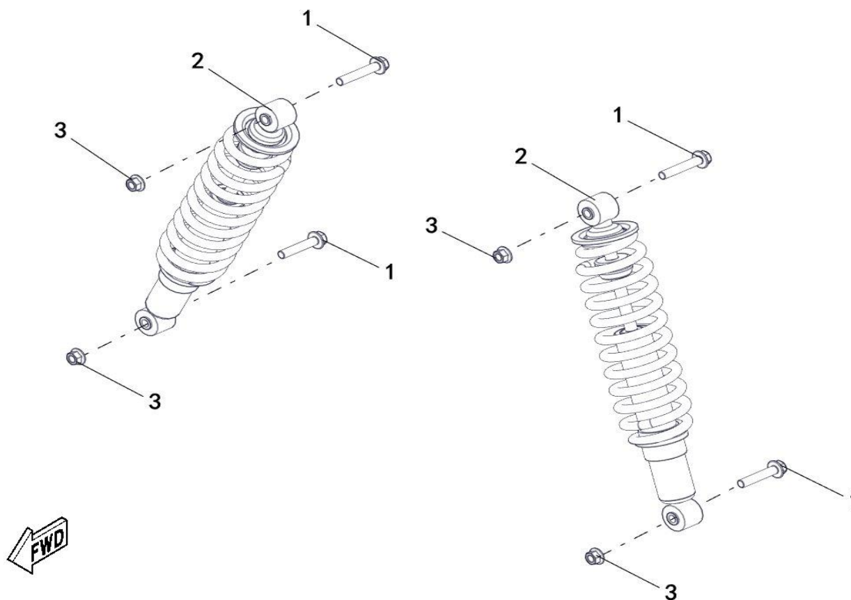
FIGUR 23 - SHOCK ABSORBER REAR (NORMAL)
