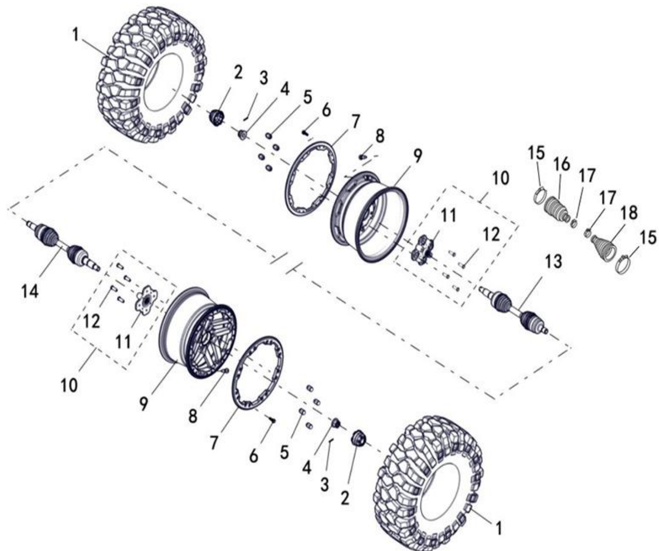
FIGUR 26 - WHEEL REAR (RIM WITH LOCK RING, TIRE 26X11-14)
