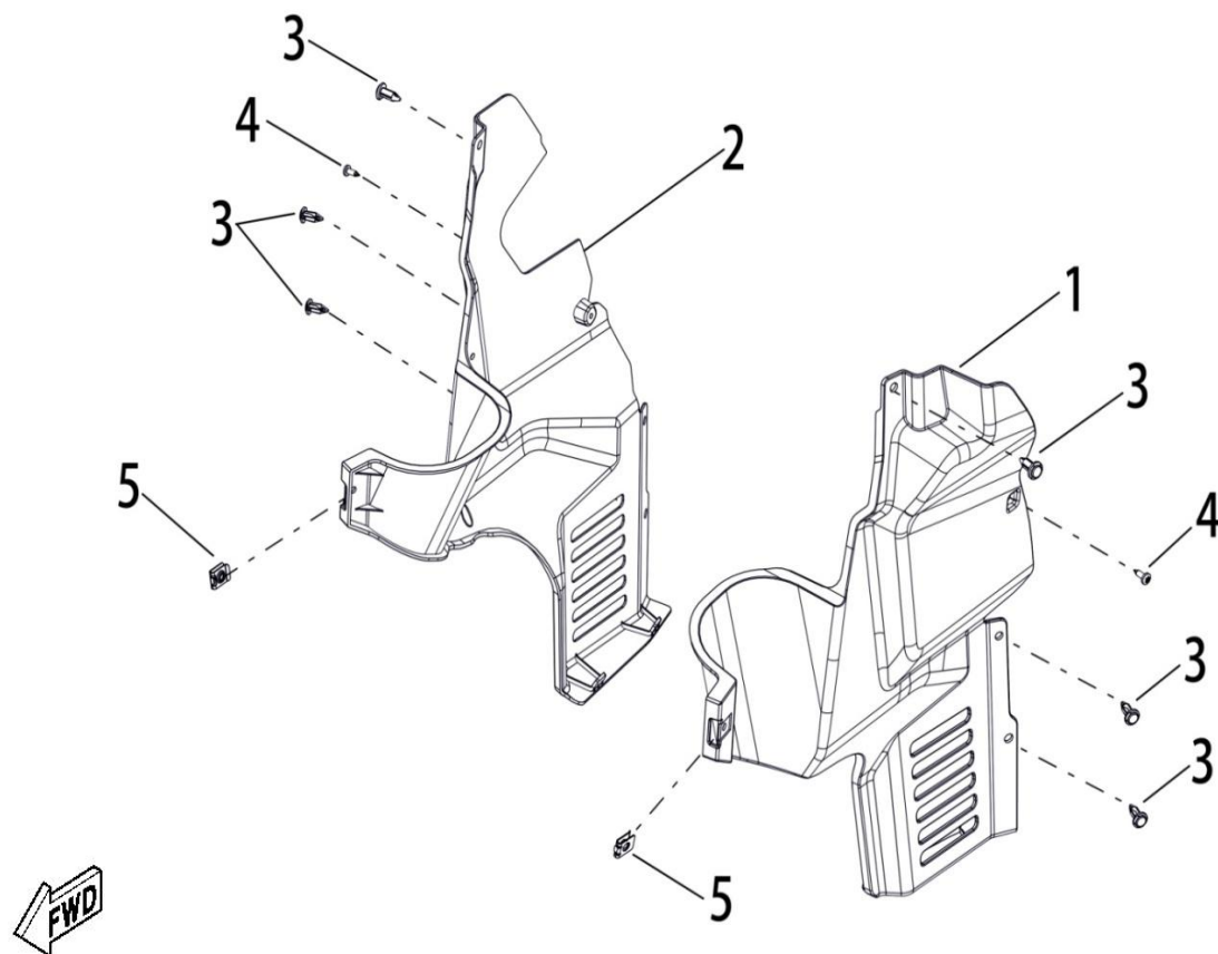
FIGUR 58 - OPTIONS (FRONT INNER FENDER)
