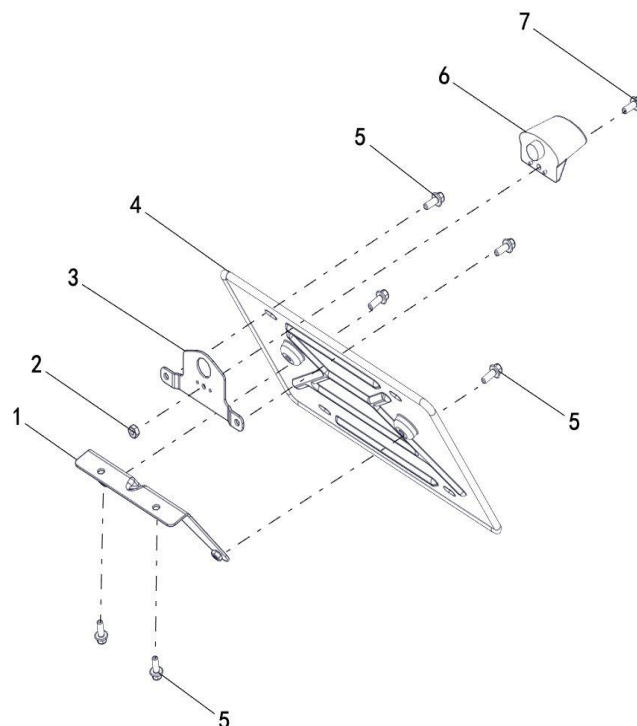
FIGUR 52 - OPTIONS (REAR LICENCE PLATE MOUNTING TO BIG REAR BUMPER)
