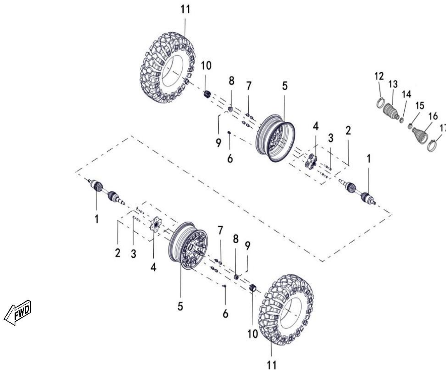
FIGUR 25 - WHEEL FRONT (NORMAL ALLOY RIM, 26X8-14)
