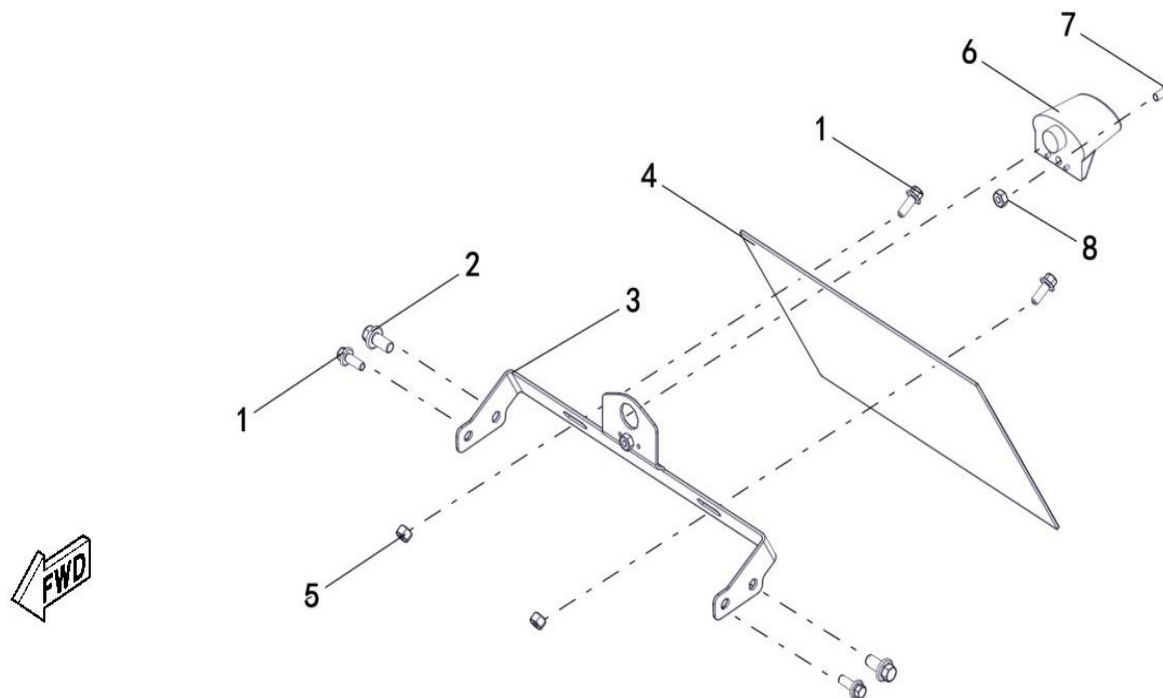
FIGUR 51 - OPTIONS (REAR LICENCE PLATE USED WITHOUT REAR BUMPER)
