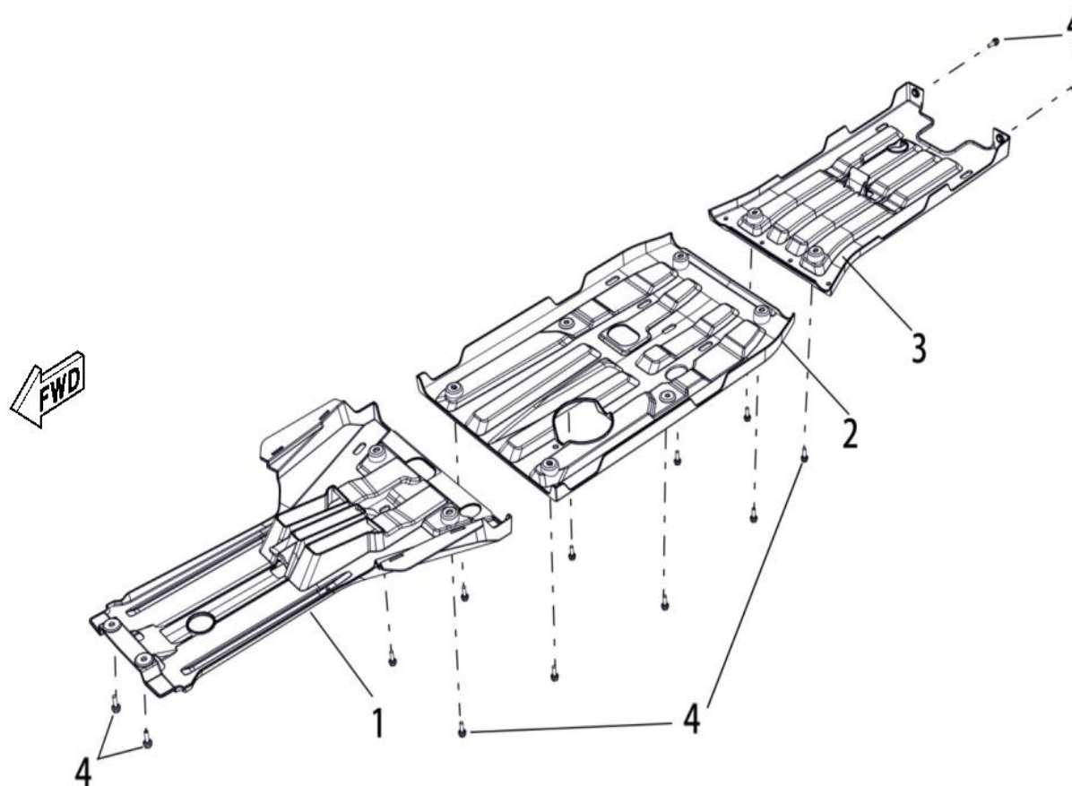
FIGUR 55 - OPTIONS (CHASSIS GUARD PLATE)
