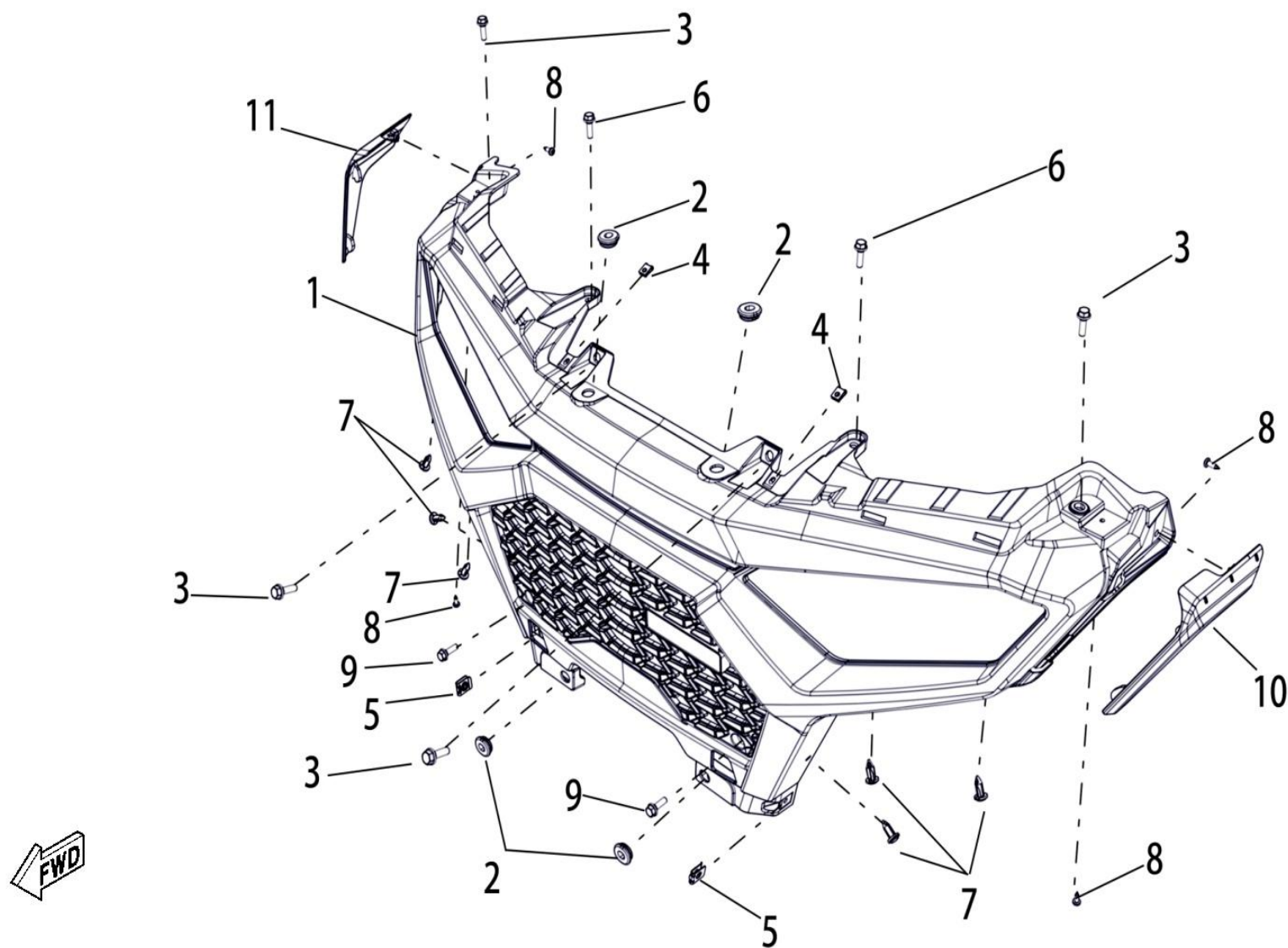
FIGUR 5 - FENDER
