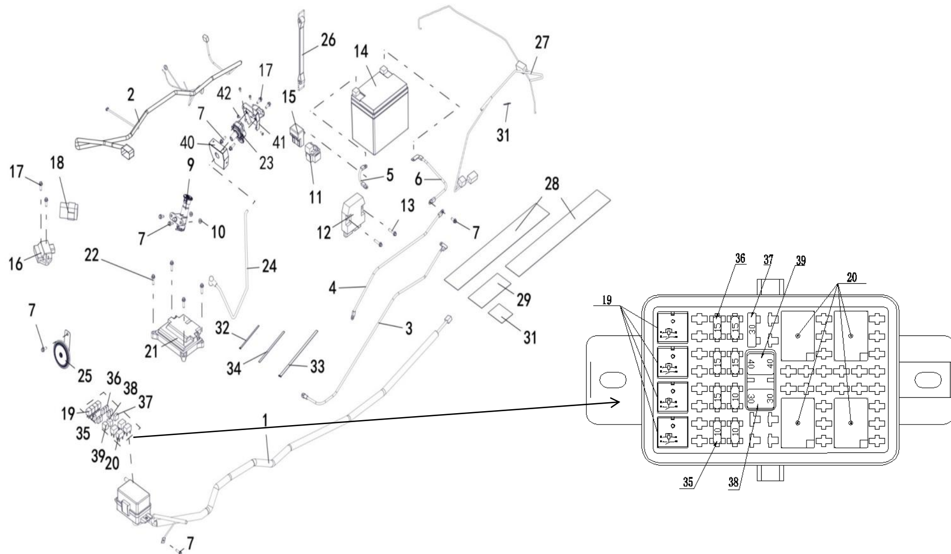
FIGUR 33 - ELECTRICAL SYSTEM
