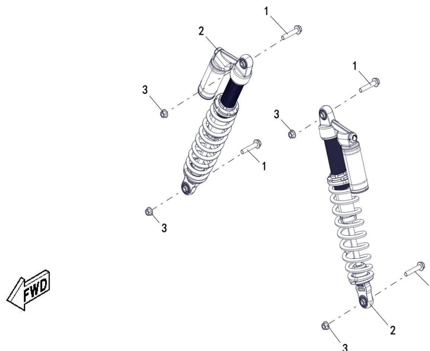
FIGUR 19 - SHOCK ABSORBER FRONT (OIL-AIR)
