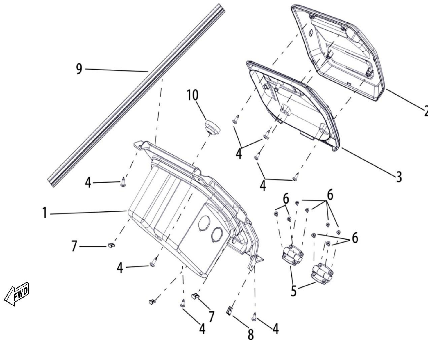
FIGUR 8 - FENDER
