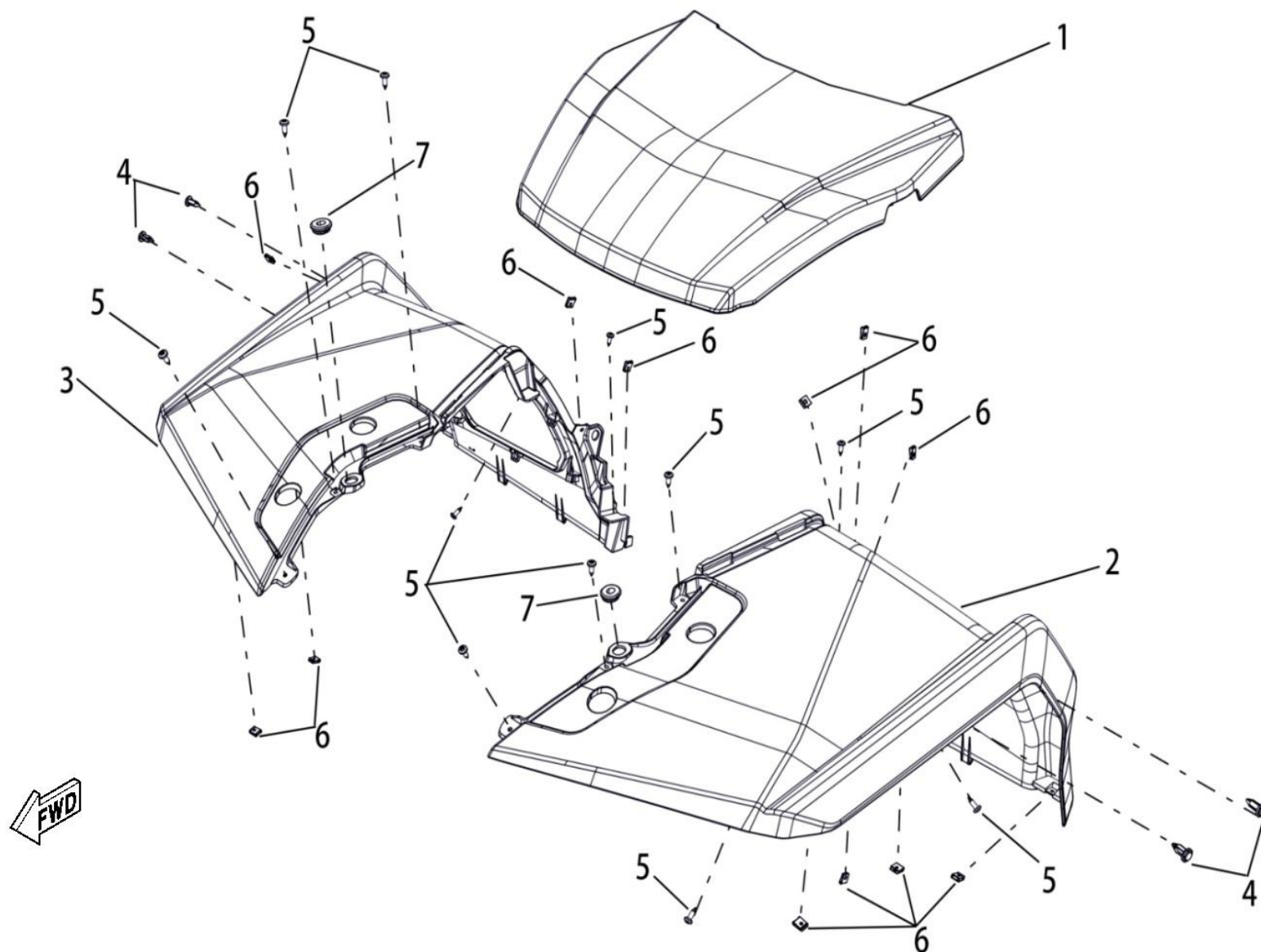
FIGUR 6 - FENDER
