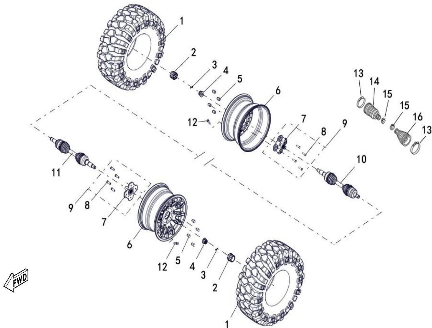
FIGUR 27 - WHEEL REAR (NORMAL ALLOY RIM, 26X10-14)
