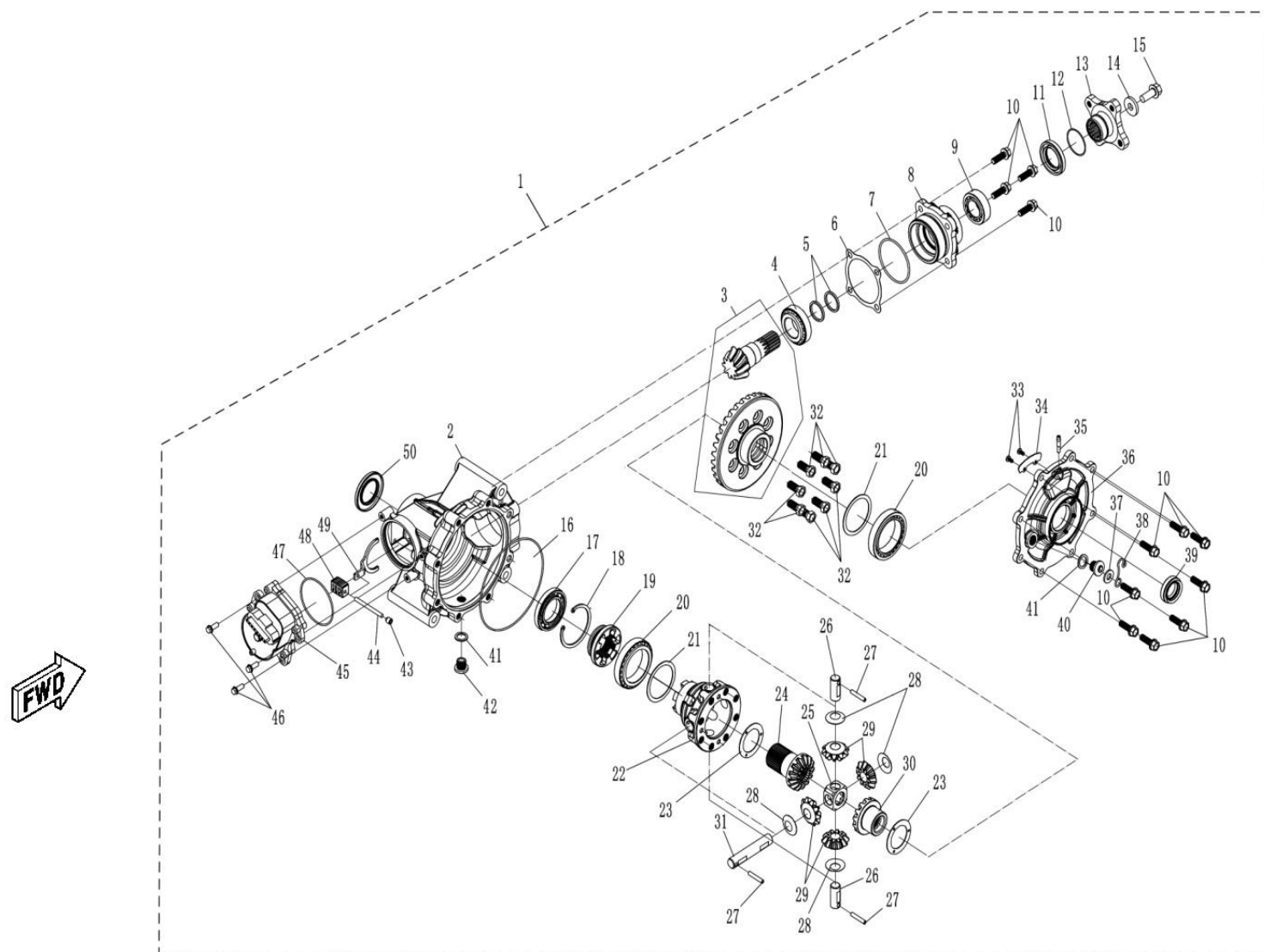
FIGUR 42 - REAR AXLE ASSY
