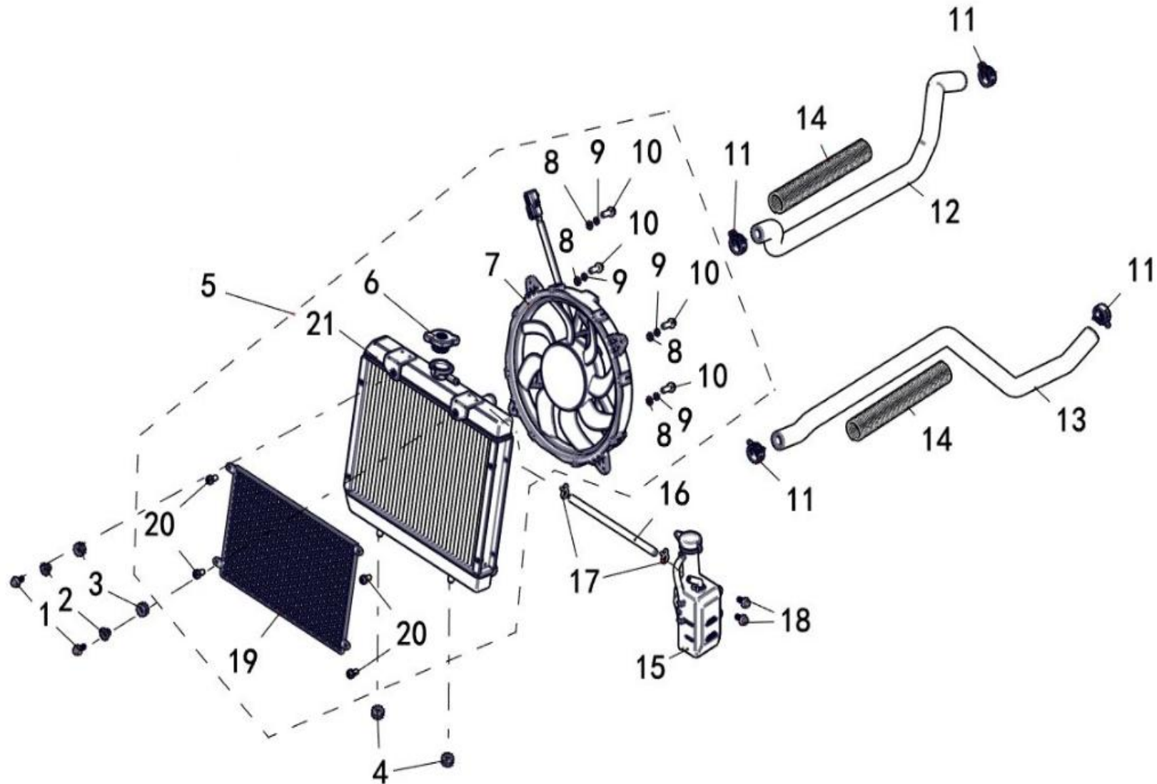
FIGUR E20 – RADIATOR
