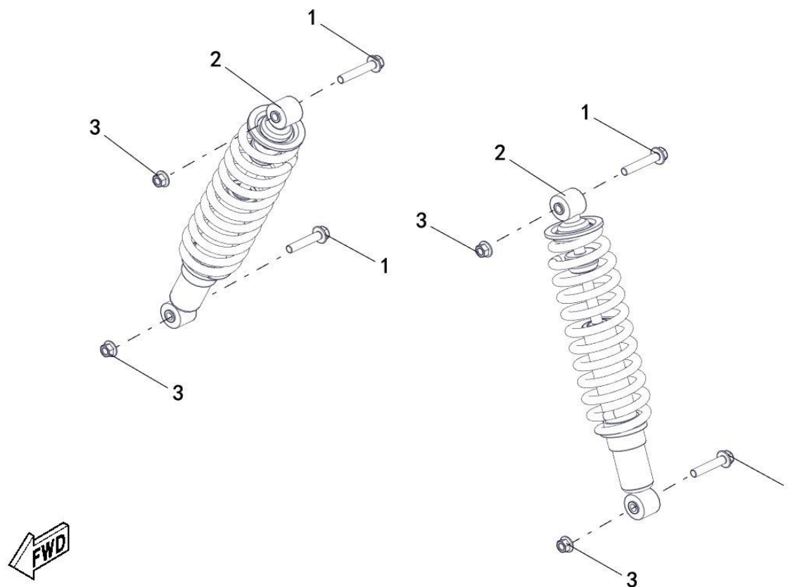
FIGUR 20 - SHOCK ABSORBER FRONT (NORMAL)
