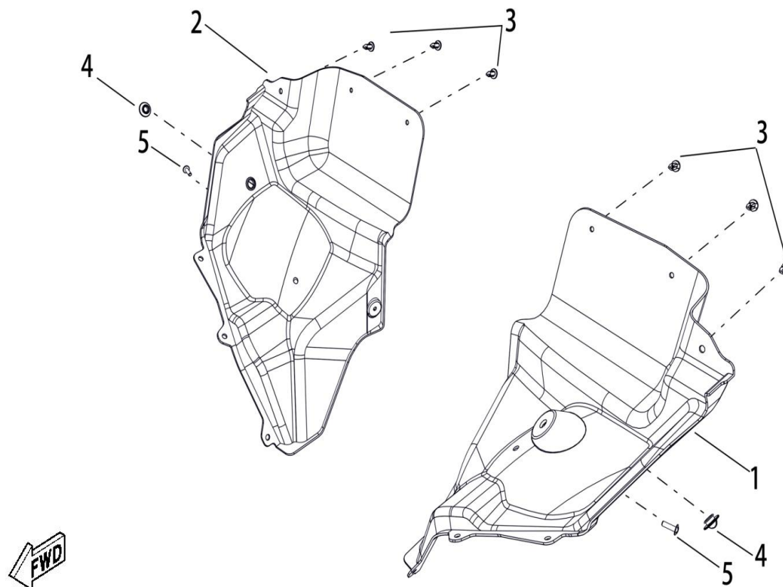
FIGUR 57 - OPTIONS (HEADLIGHT SHIELD)
