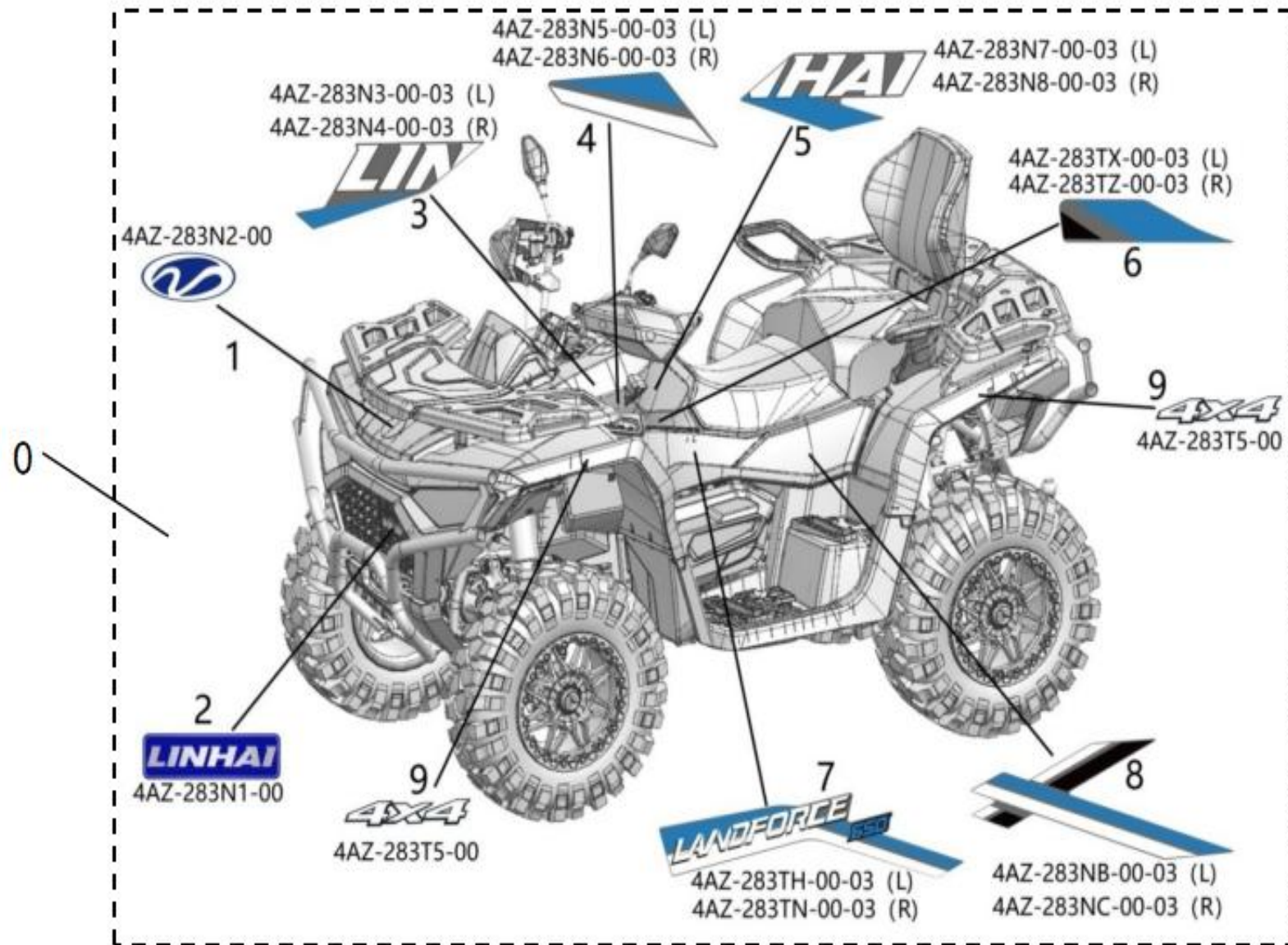
FIGUR 66 -DECALS (LINHAI LOGO) (MATCH DARK GRAY FENDES)
