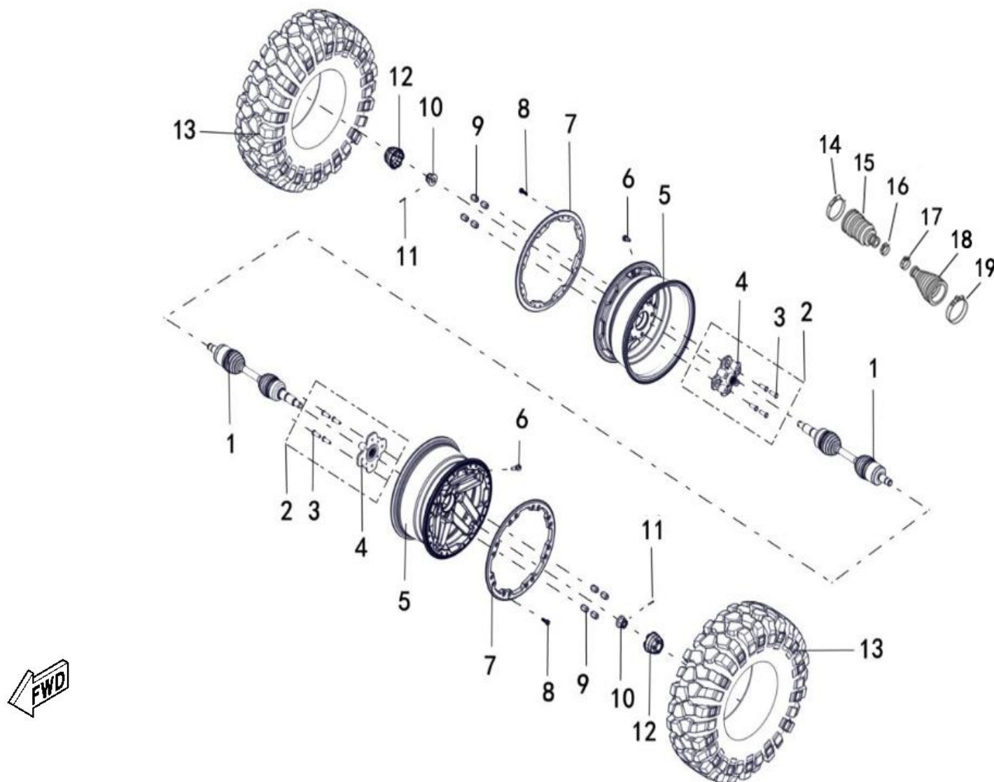
FIGUR 24 - WHEEL FRONT (RIM WITH LOCK RING, TIRE 26X9-14)
