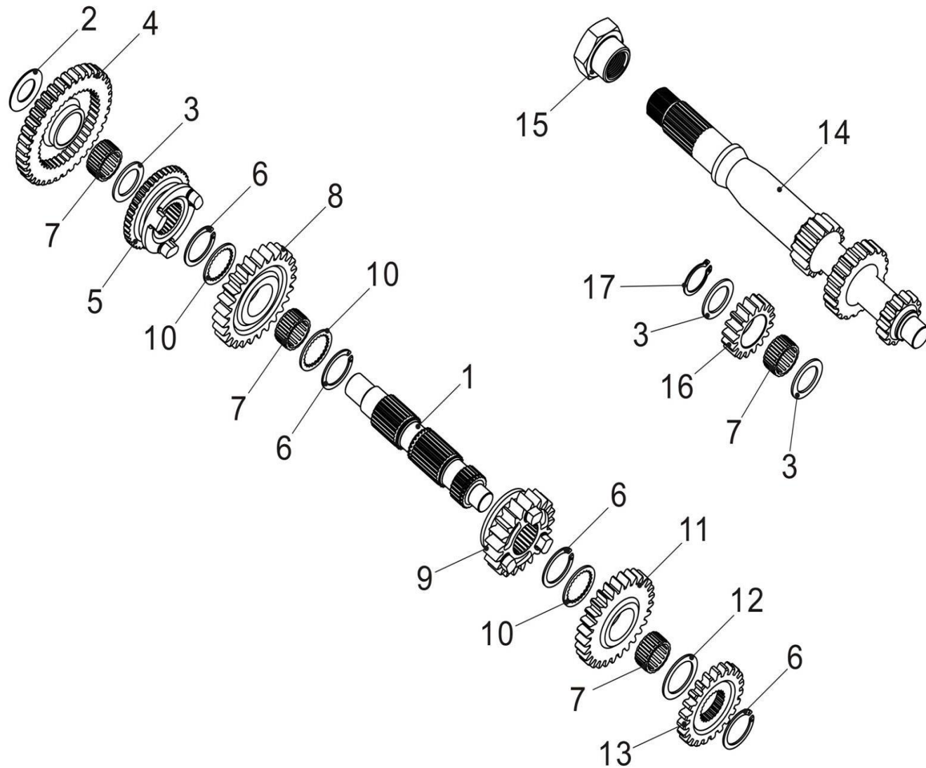
FIGUR E14 - TRANSMISSION I
