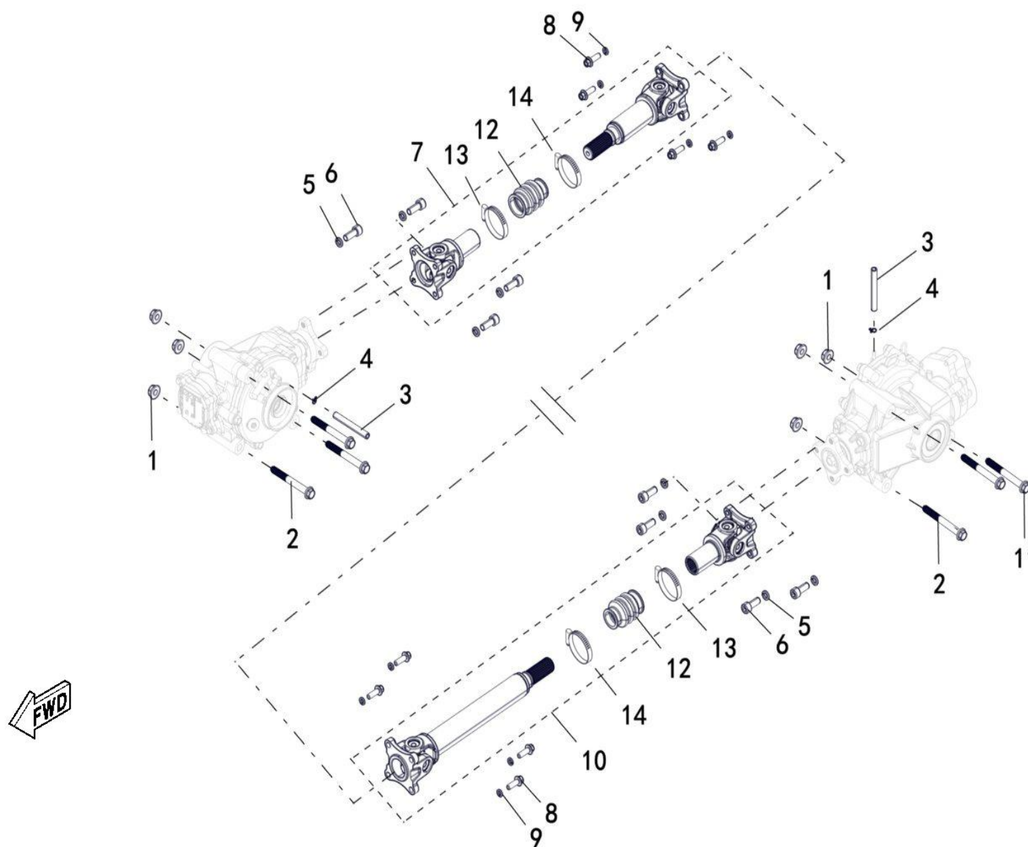
FIGUR 30 - FRONT AND REAR KNUCKLE ASSY
