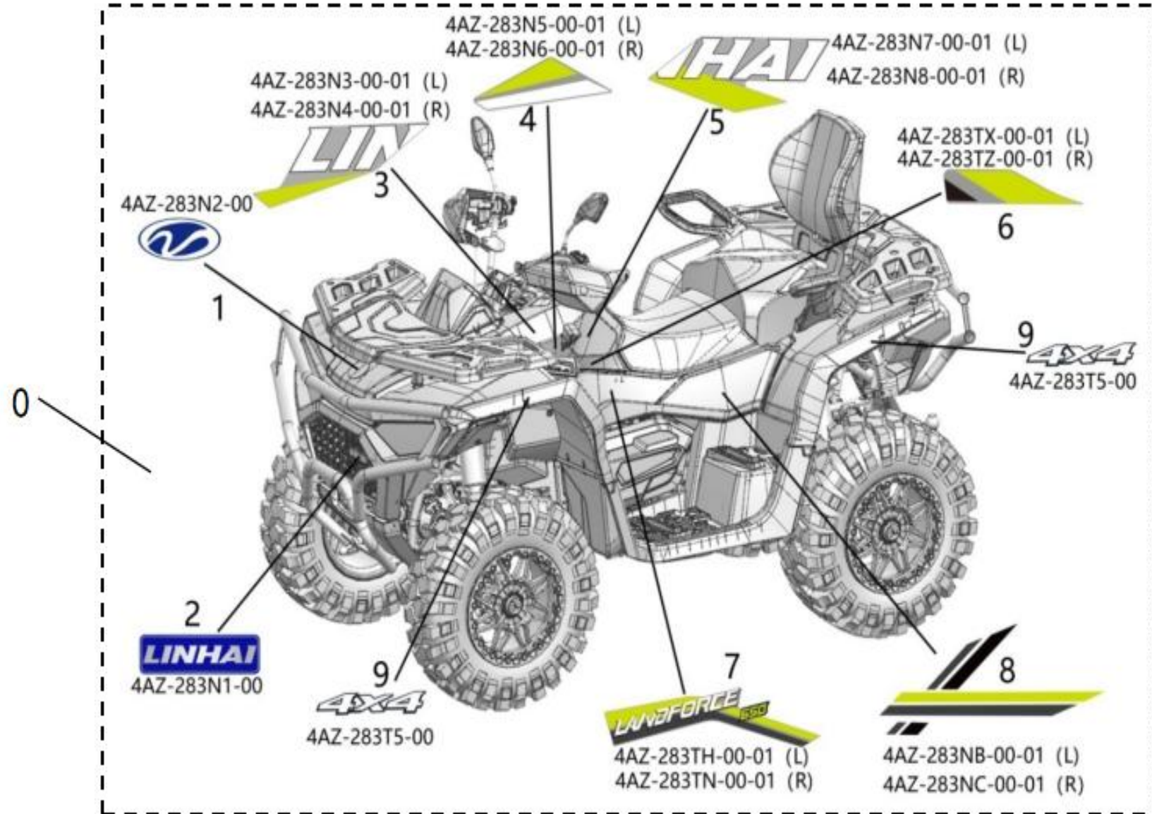
FIGUR 64 - DECALS (LINHAI LOGO) (MATCH LIGHT GRAY FENDES)
