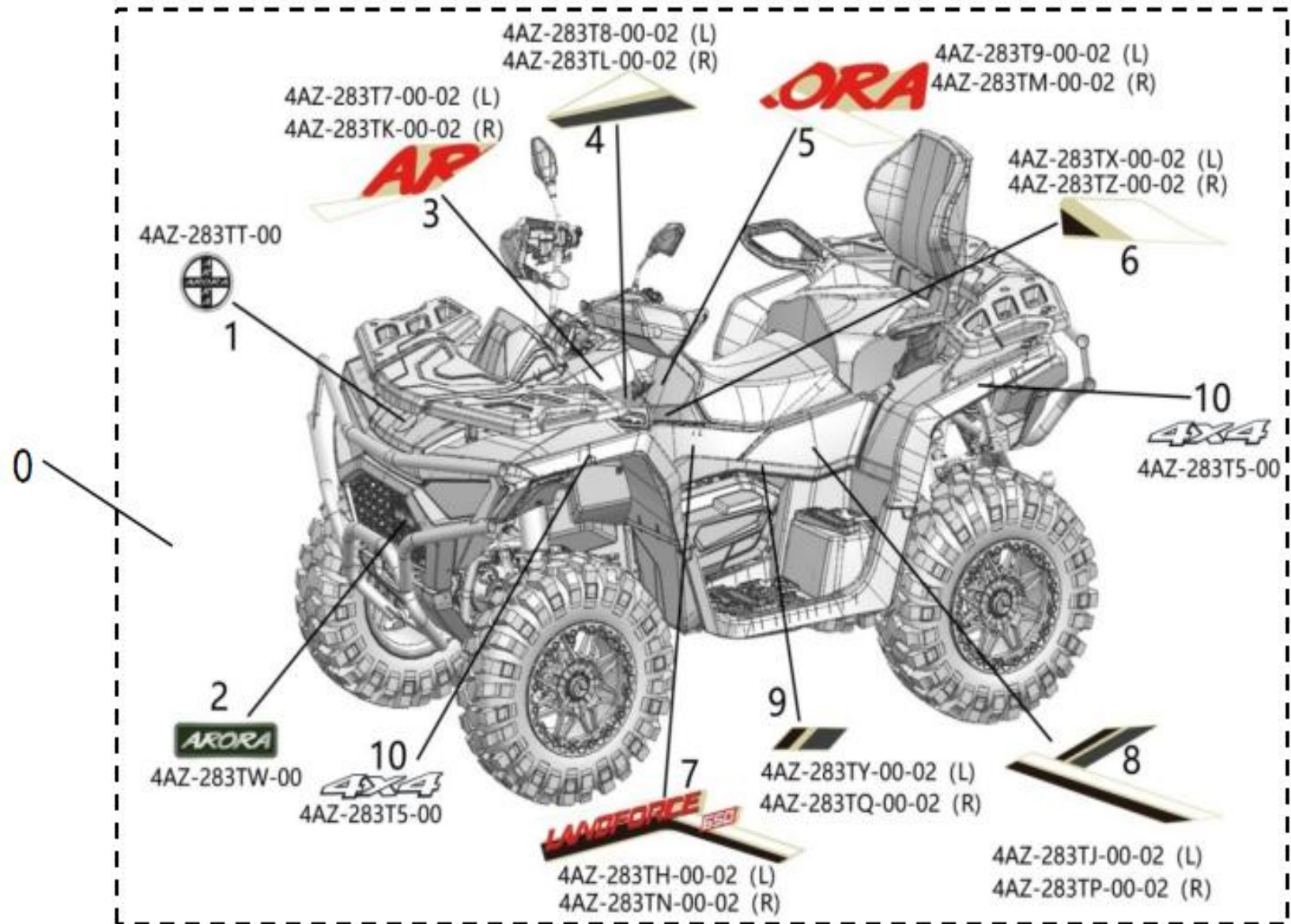
FIGUR 60 - DECALS (ARORA LOGO) (MATCH GOLD FENDES)
