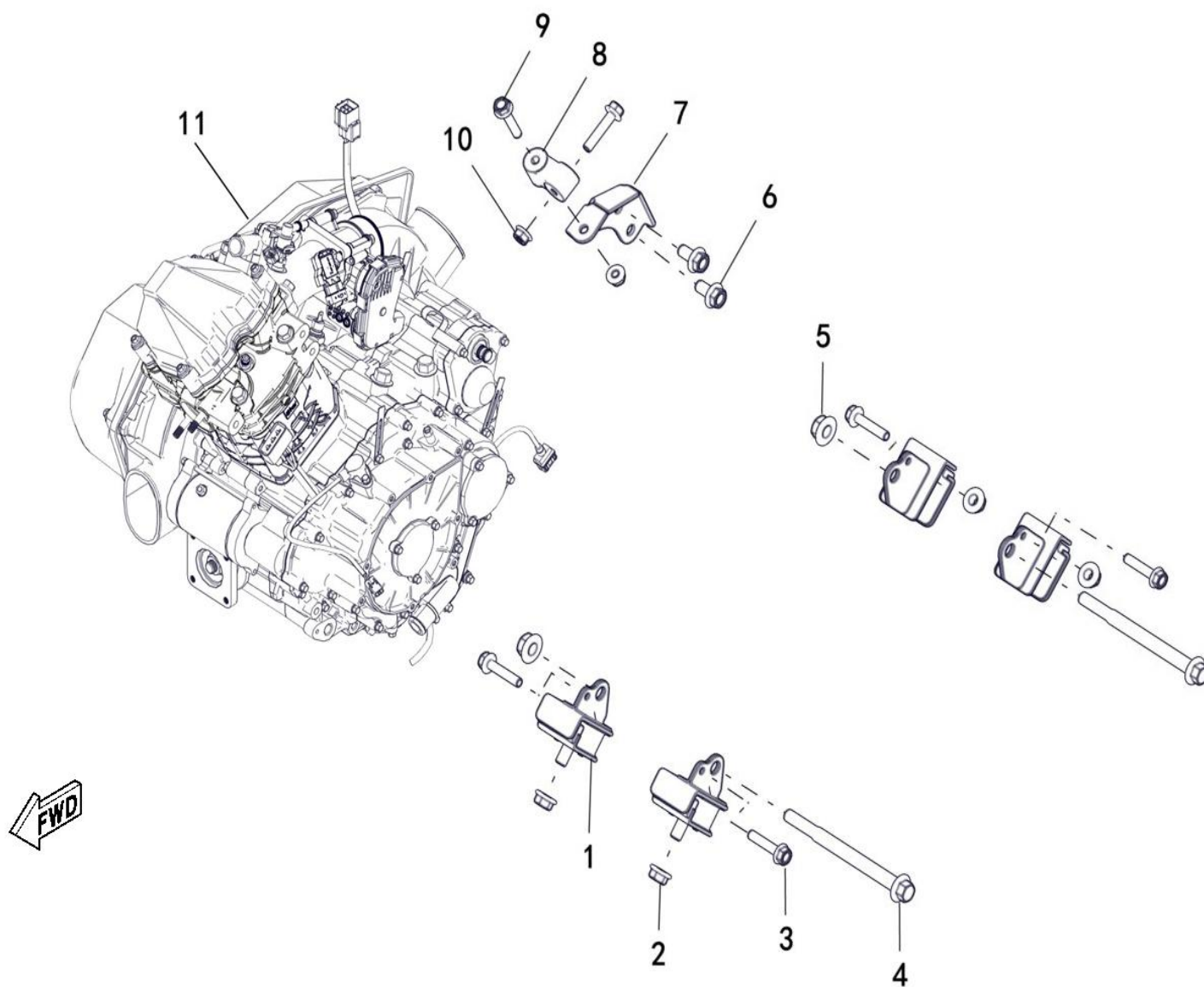
FIGUR 43 - GEARBOX INSTALLATION
