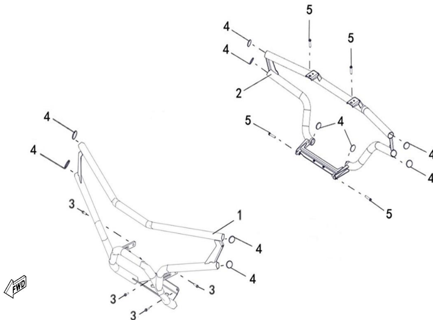
FIGUR 38 - BUMPER (BIG)
