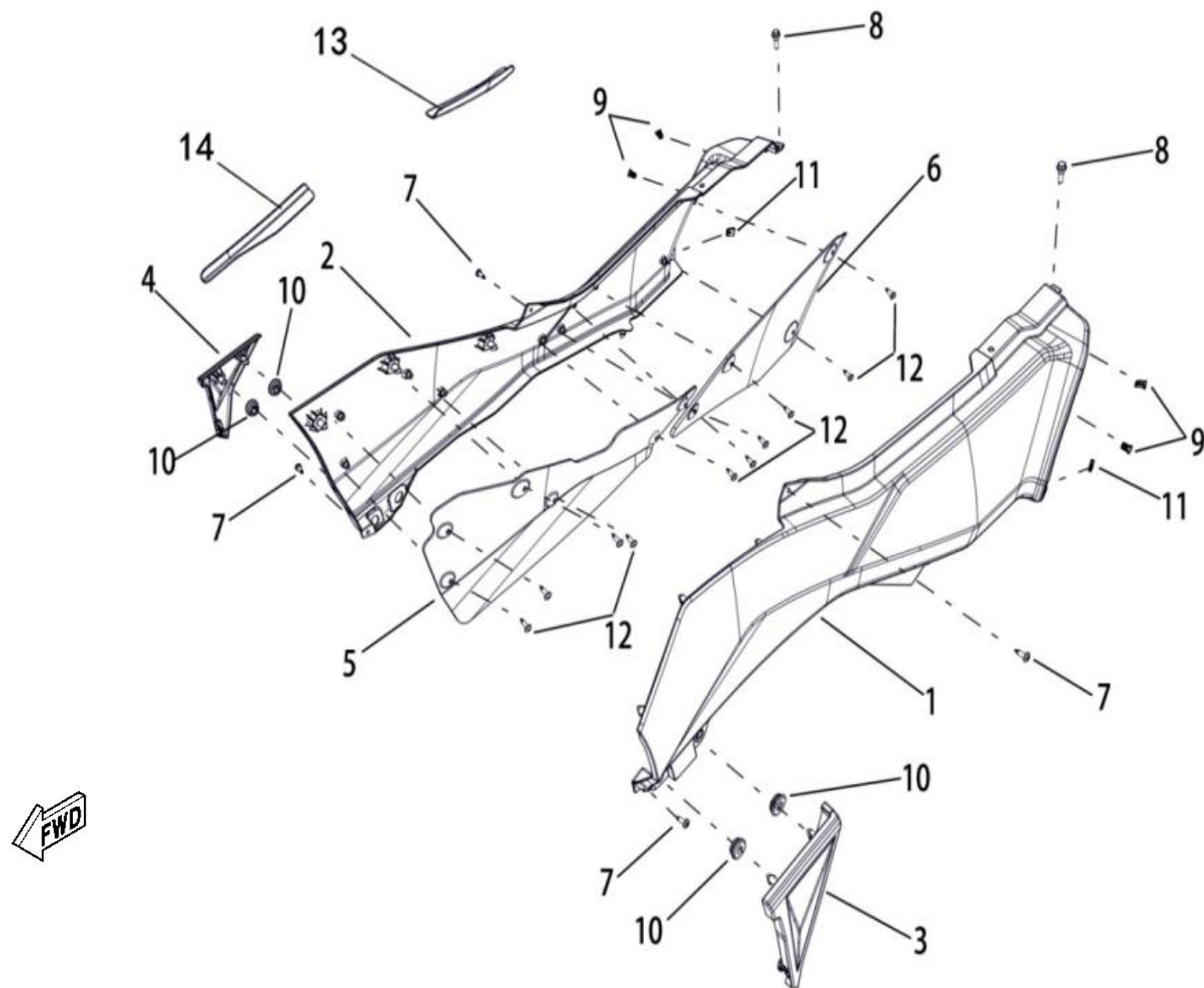
FIGUR 10 - FENDER
