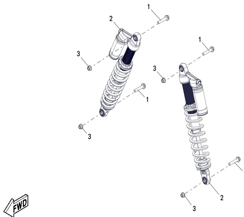
FIGUR 22 - SHOCK ABSORBER REAR (OIL-AIR)
