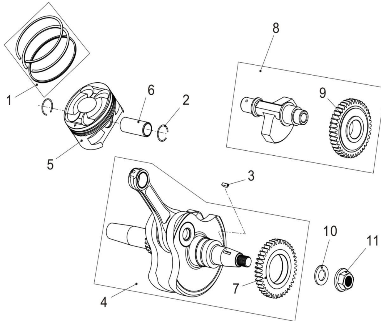
FIGUR E5 - CRANKSHAFT COMP
