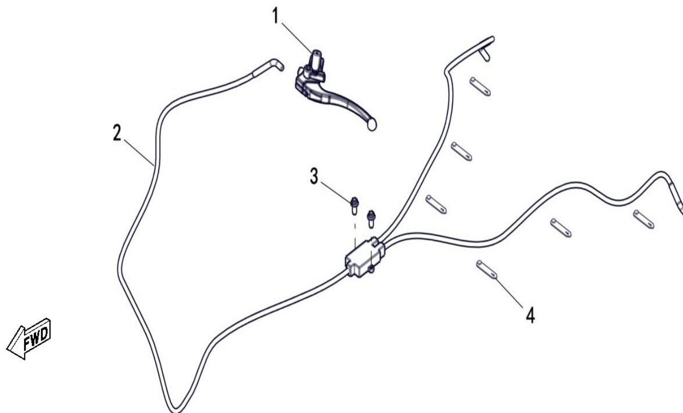
FIGUR 37 - AUXILIARY BRAKE
