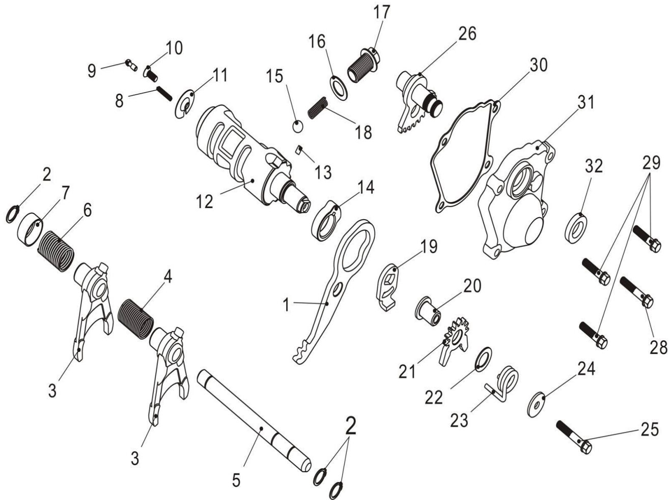
FIGUR E16 - TRANSMISSION III
