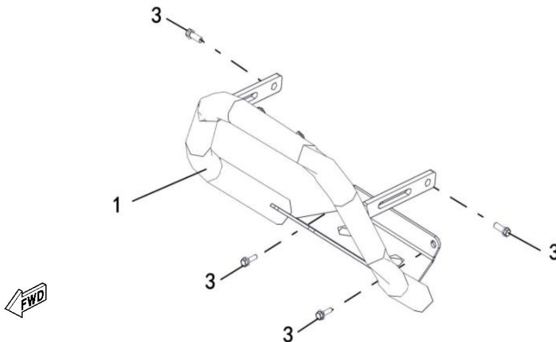
FIGUR 39 - BUMPER (SMALL)
