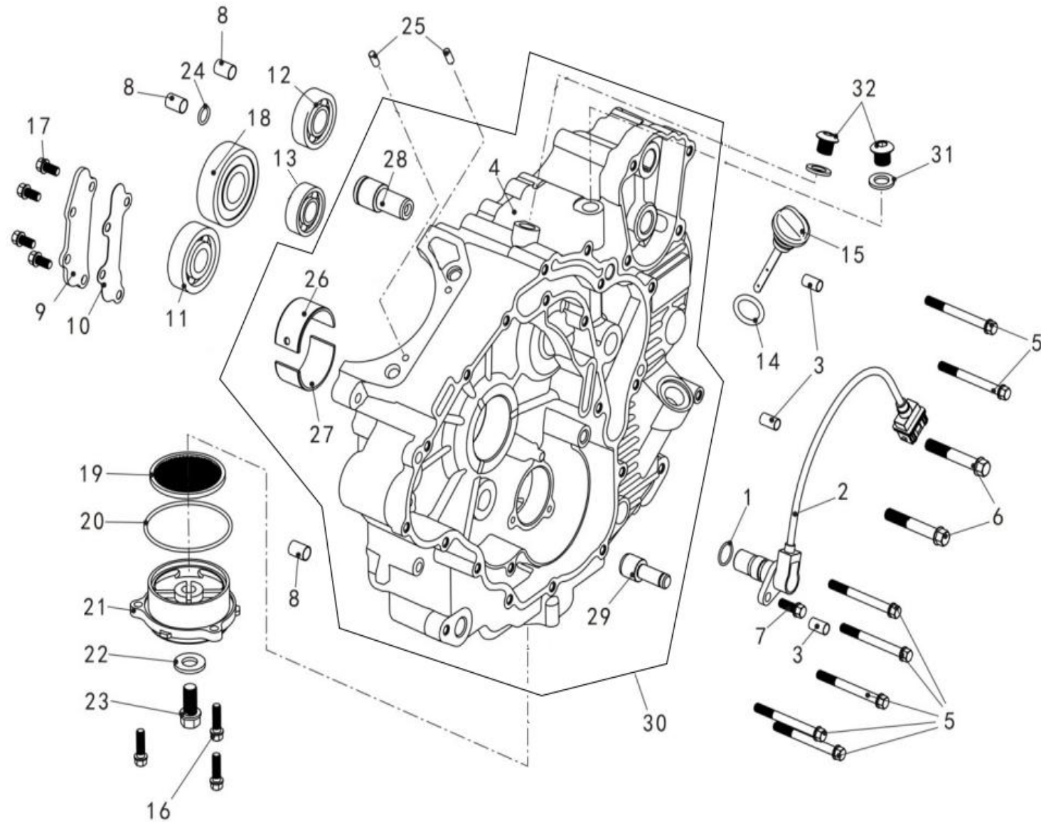
FIGUR E6 - LEFT CRANKCASE
