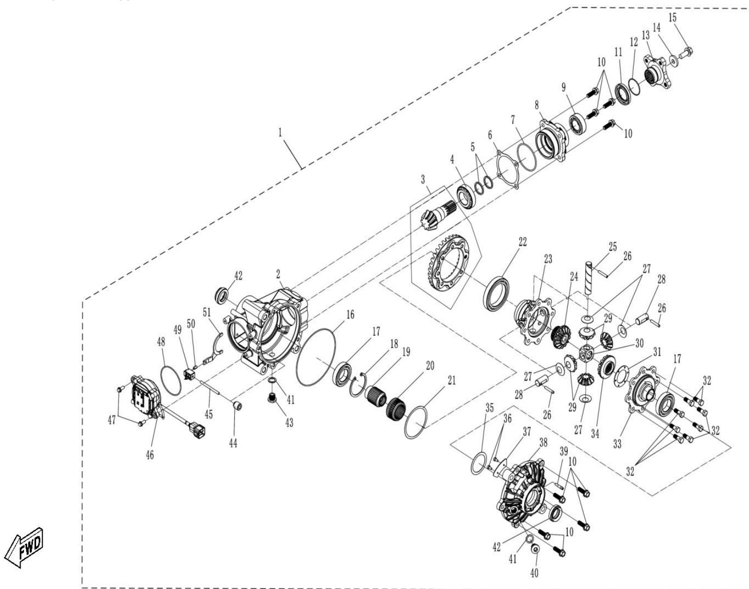
FIGUR 41 - FRONT AXLE ASSY
