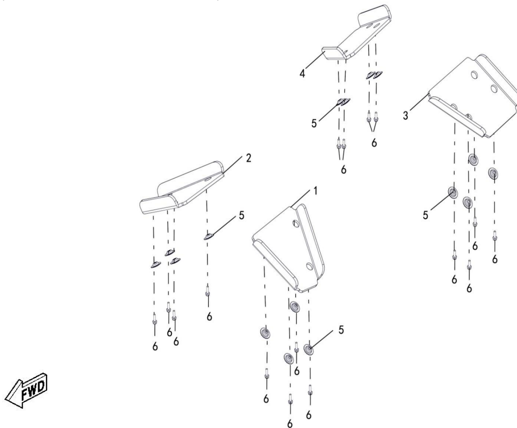
FIGUR 48 - OPTIONS (LOWER A-ARM BOARD GUARD ASSY)
