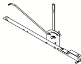
Hopper Assembly 1pc
