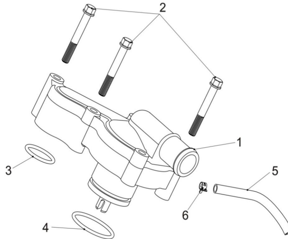
FIGUR 18 – VANDPUMPE / WATER PUMP
