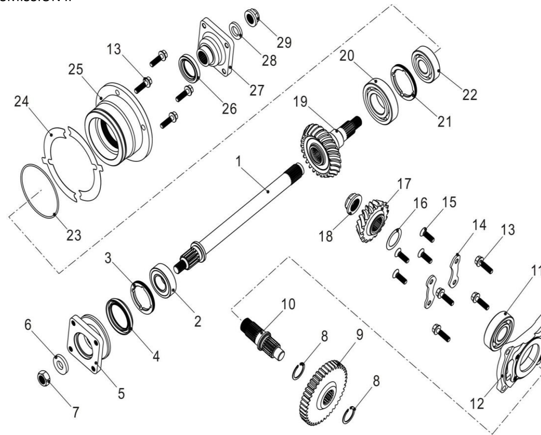
DELE TIL FIG 15 (TRANSMISSION II / TRANSMISSION II)
