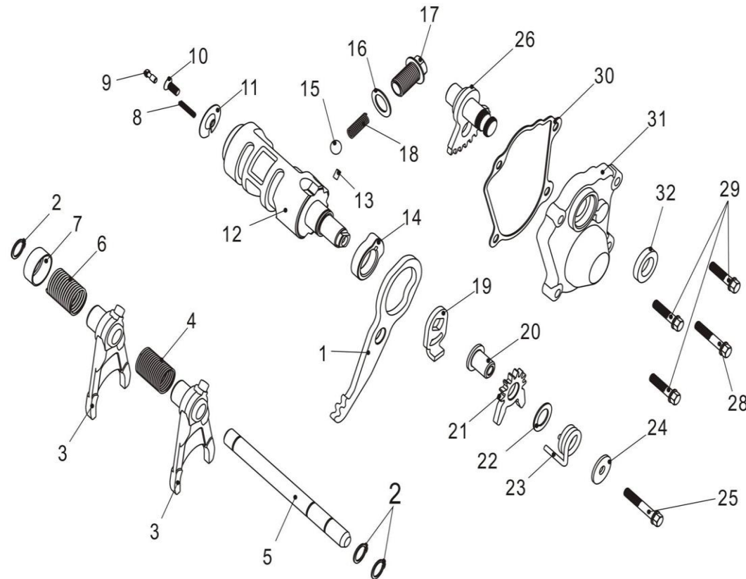
DELE TIL FIG 16 (TRANSMISSION III / TRANSMISSION III)
