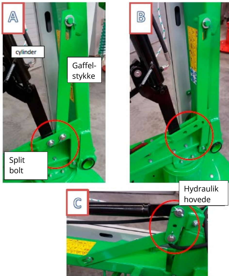
Figure 7 A) B) C) Assembly of the mower
