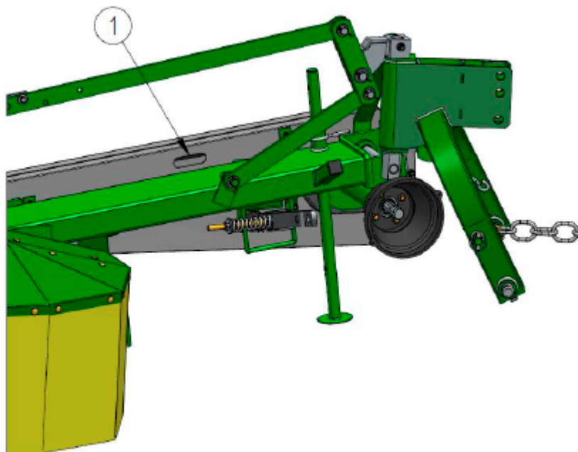
Figure 23 Checking of the proper adjustment of V-belts tension: 1) inspection opening for checking the tension of the belts
