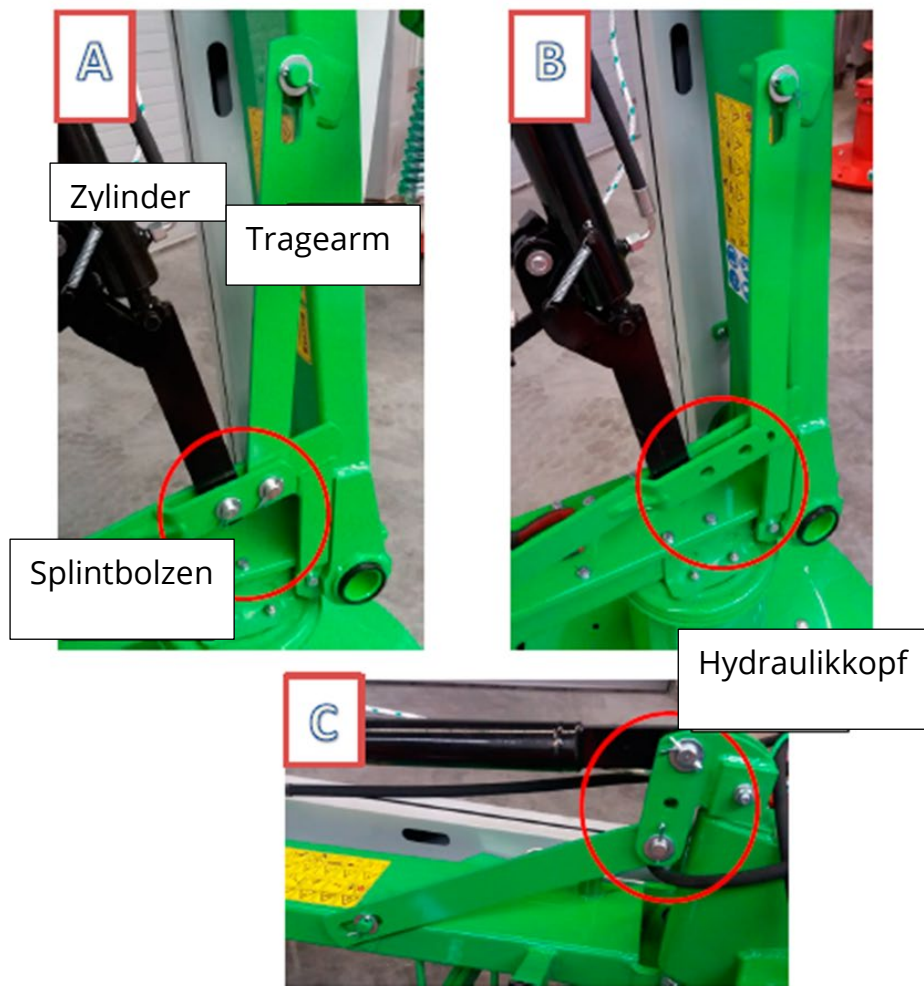
Figure 7 A) B) C) Assembly of the mower
