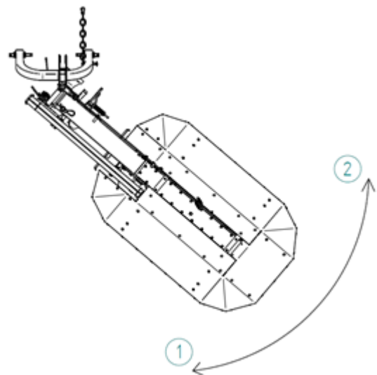
1=Transportposition 2=Driftsposition
