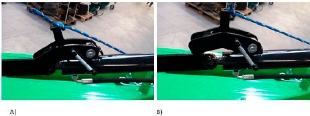
Figure 15 Locking the cylinder: A) locked, B) open
