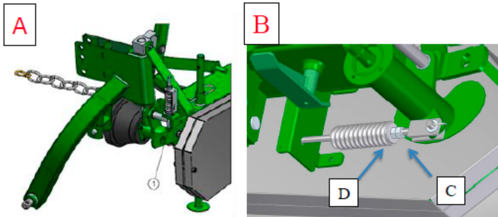
Figure 22 Adjustment of the V-belts tension: A) Belt tensioner B) for Eco CUT 210 version
