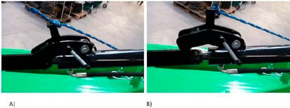
Figure 15 Locking the cylinder: A) locked, B) open
