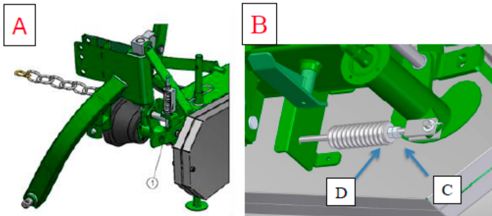
Figure 22 Adjustment of the V-belts tension: A) Belt tensioner B) for Eco CUT 210 version
