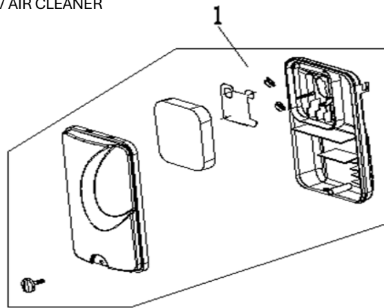
MOTOR FIGUR 10 – LUFTFILTER / AIR CLEANER
