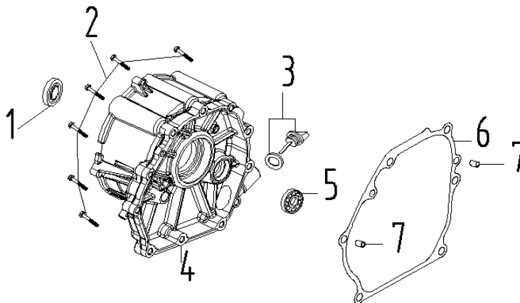
MOTOR FIGUR 3 – KRUMTAPDÆKSEL / CRANKCASE COVER
