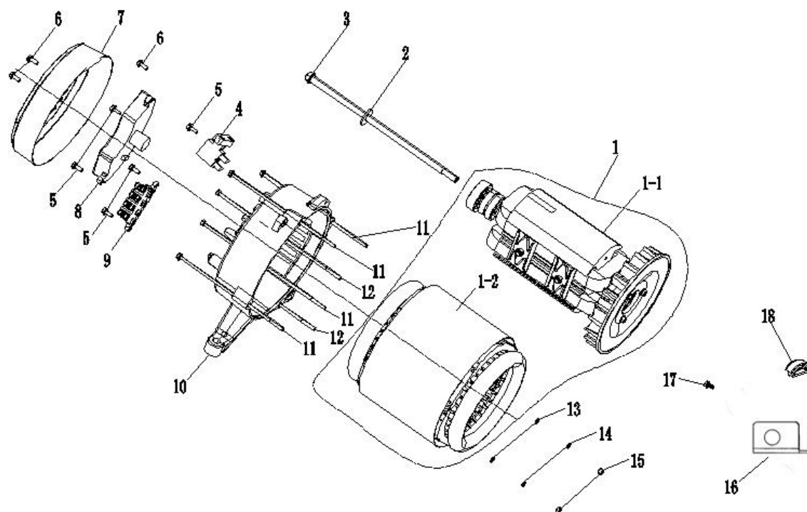
FIGUR 3 – MOTOR / ENGINE
