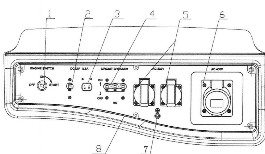
FIGUR 5 – KONTROL PANEL / CONTROL PANEL
