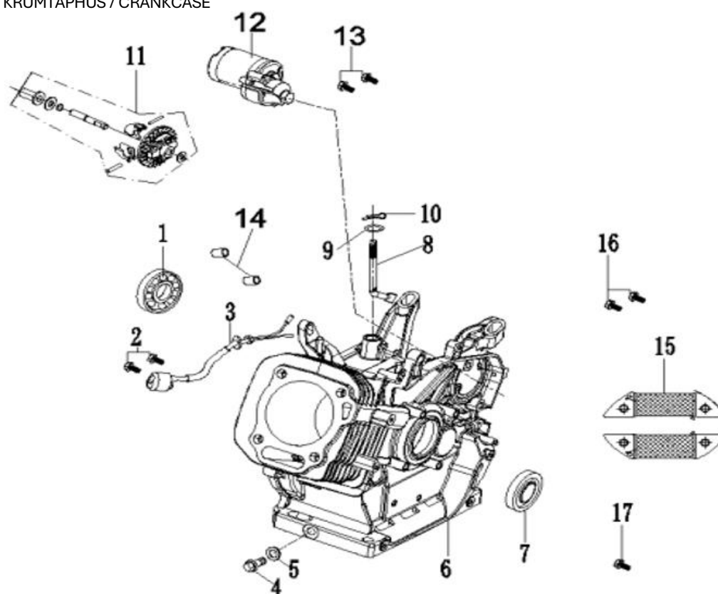
MOTOR FIGUR 2 – KRUMTAPHUS / CRANKCASE
