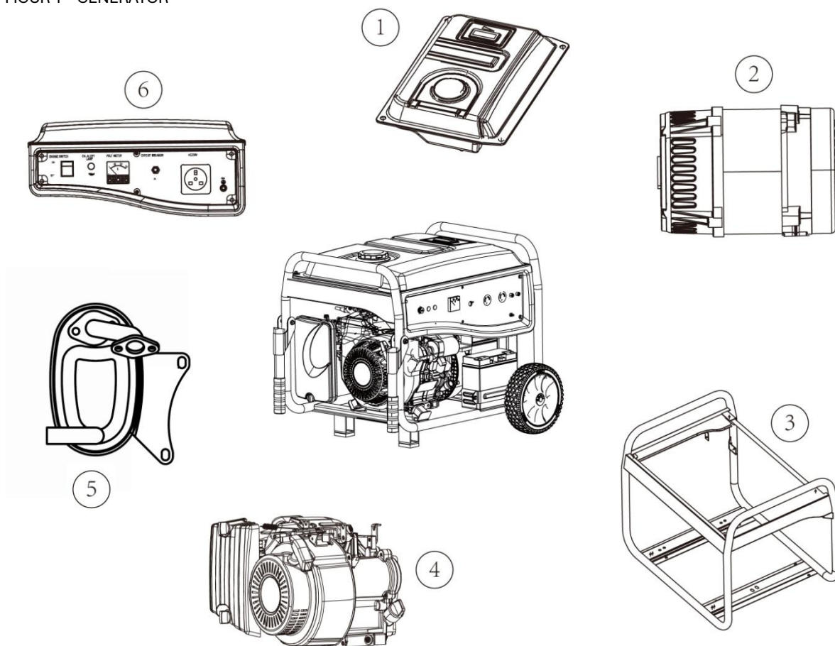
FIGUR 1 – GENERATOR
