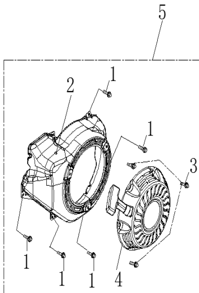
MOTOR FIGUR 7 – REKYLSTART / RECOIL STARTER
