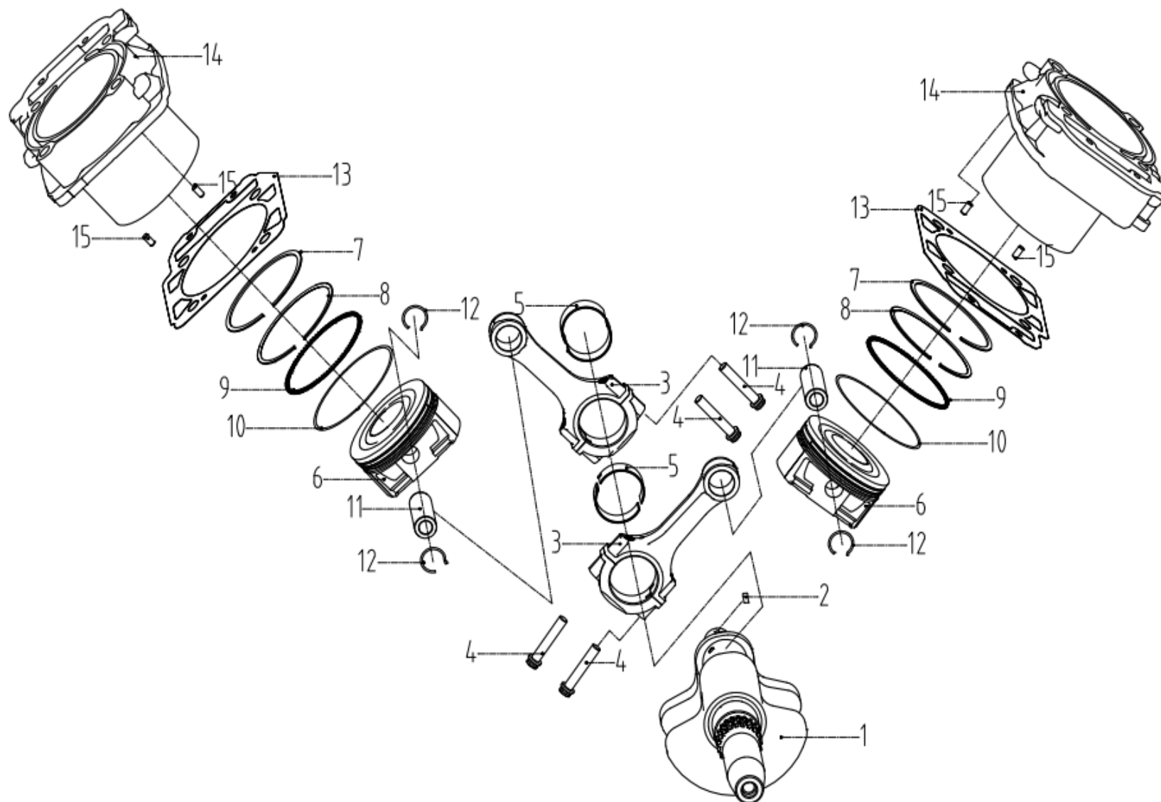
FIGUR 4 – KRUMTAP, STEMPEL &amp; CYLINDER / CRANKSHAFT, PISTON &amp; CYLINDER
