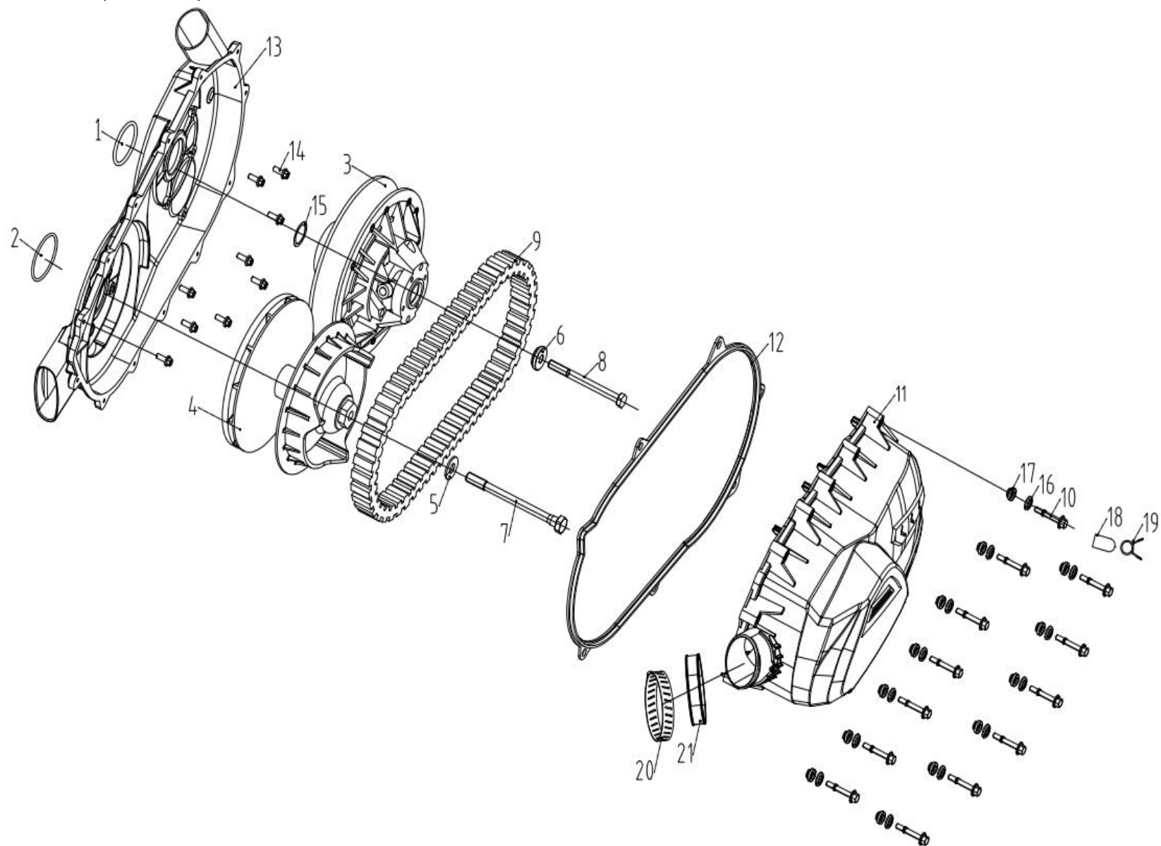
FIGUR 11 – CVT-KOBLING, DRIVREM / CVT-TRANSMISSION
