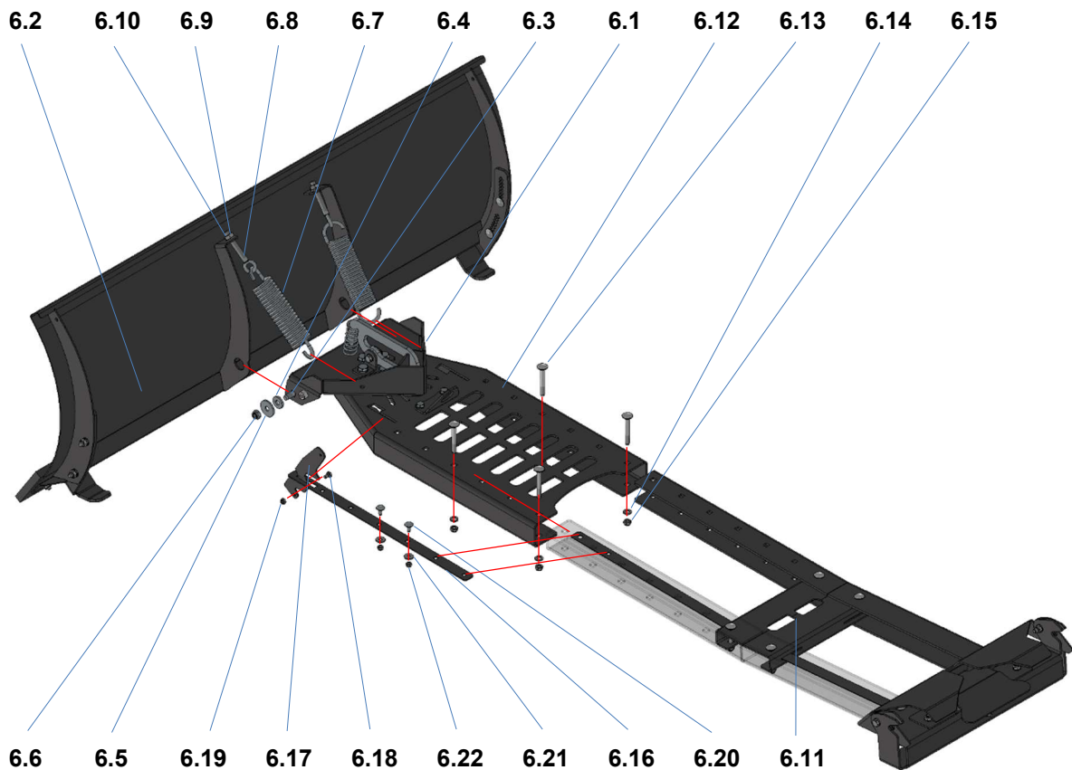
BILD. 6: Snowblade-Montage
