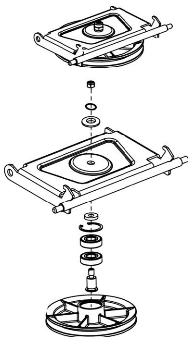
POS G17 VARIATOR SKIVE
