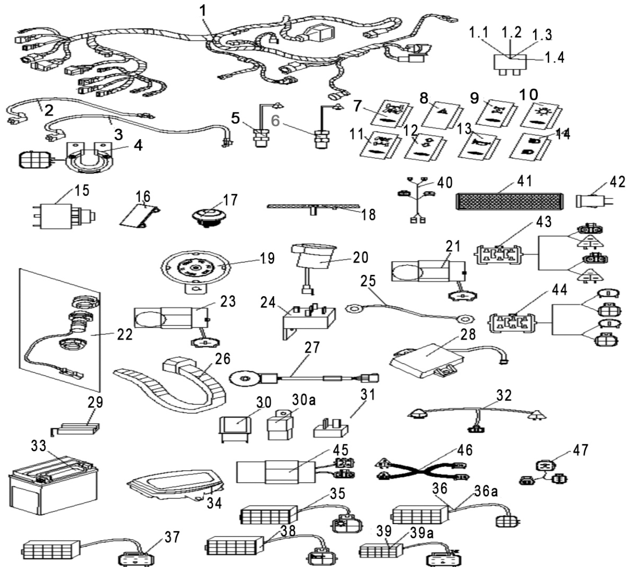
FIGUR 18 – ELEKTRISK SYSTEM &amp; LYGTER / ELECTRICAL SYSTEM &amp; LIGHTS
