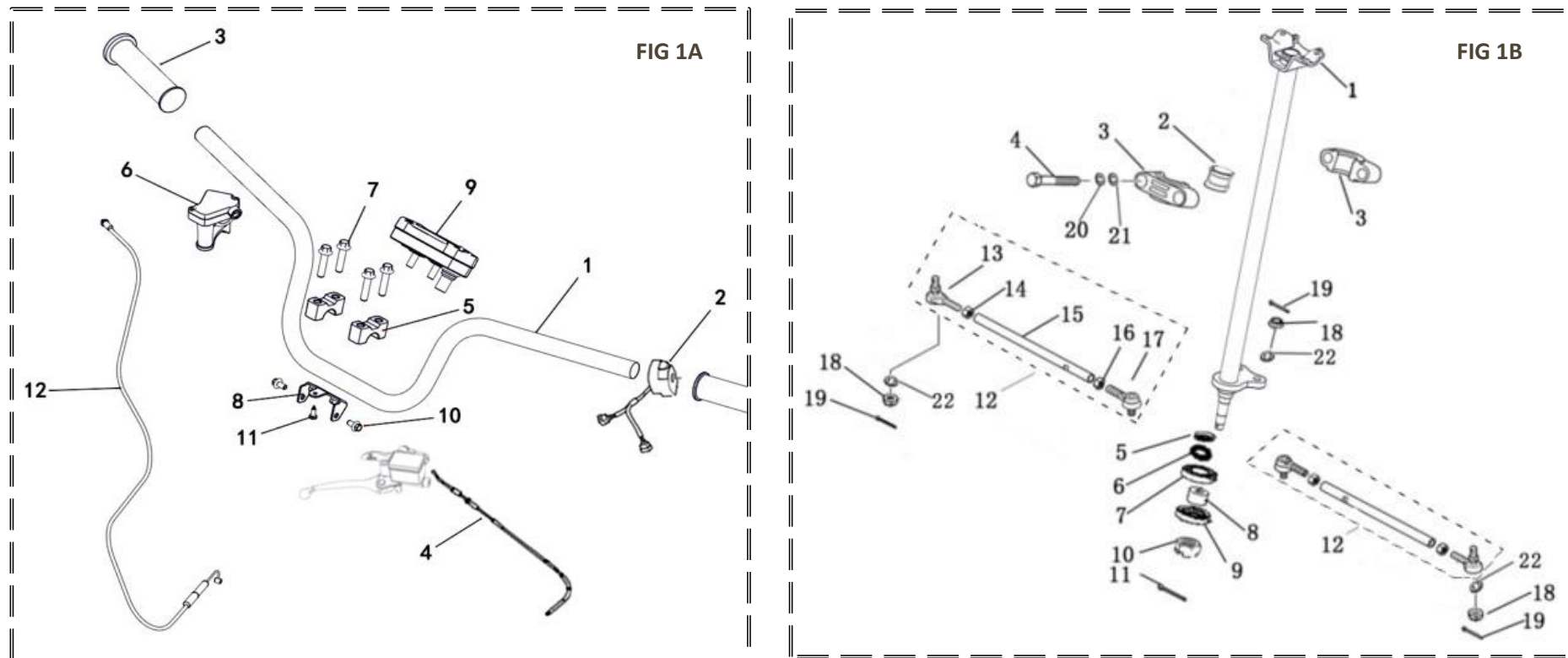
FIGUR 1 – STYR / HANDLEBAR
