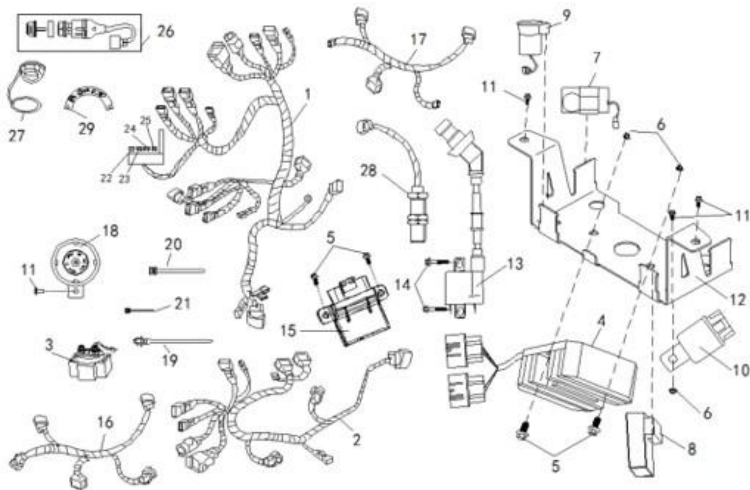
FIGUR 12 – ELEKTRISK SYSTEM / ELECTRICAL SYSTEM
