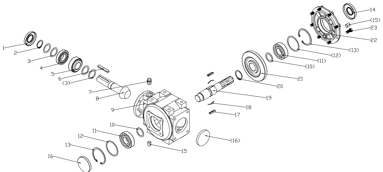
FIG. 3 GEARBOX COMPONENTS
