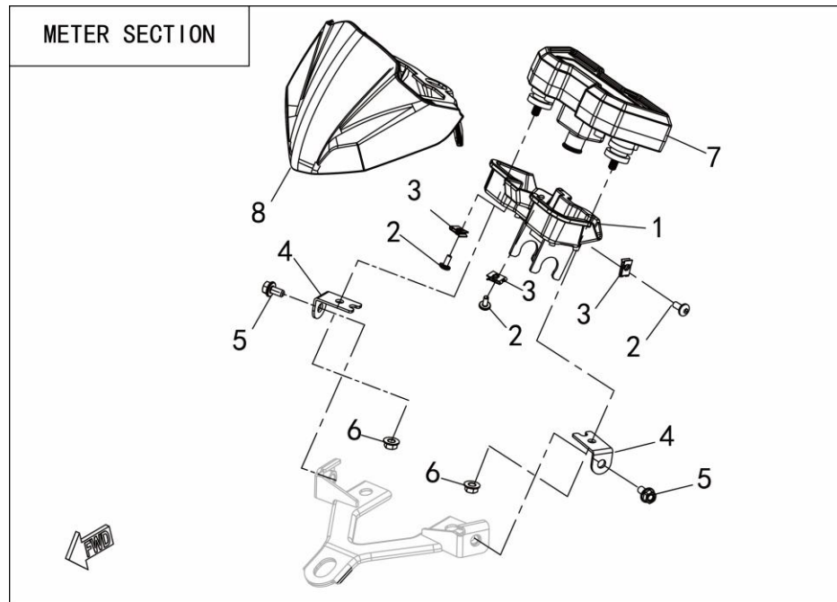
FIGUR 20 – INSTRUMENT
