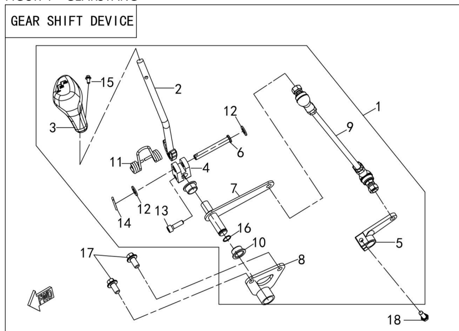
FIGUR 4 – GEARSTANG
