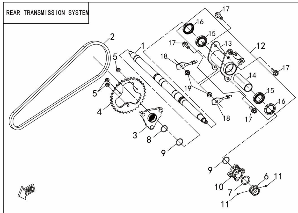
FIGUR 6 – GEARKASSE
