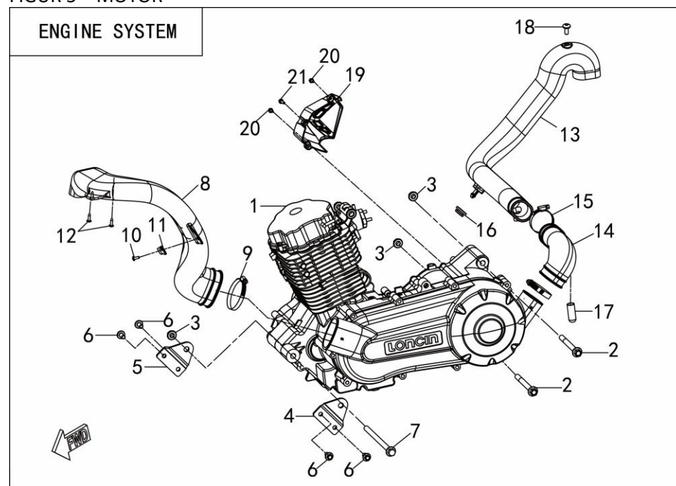
FIGUR 5 – MOTOR
