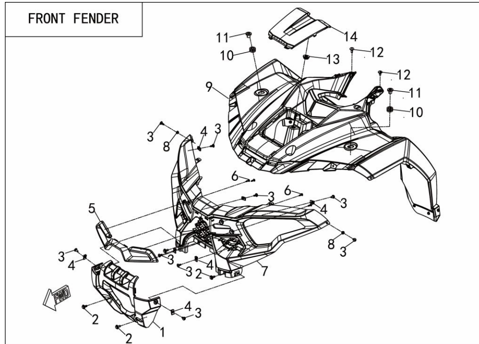
FIGUR 19 – FOR KOFANGER
